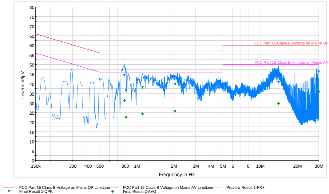
Plot 7-6. Line Conducted Plot (LN) – Battery at 100%
