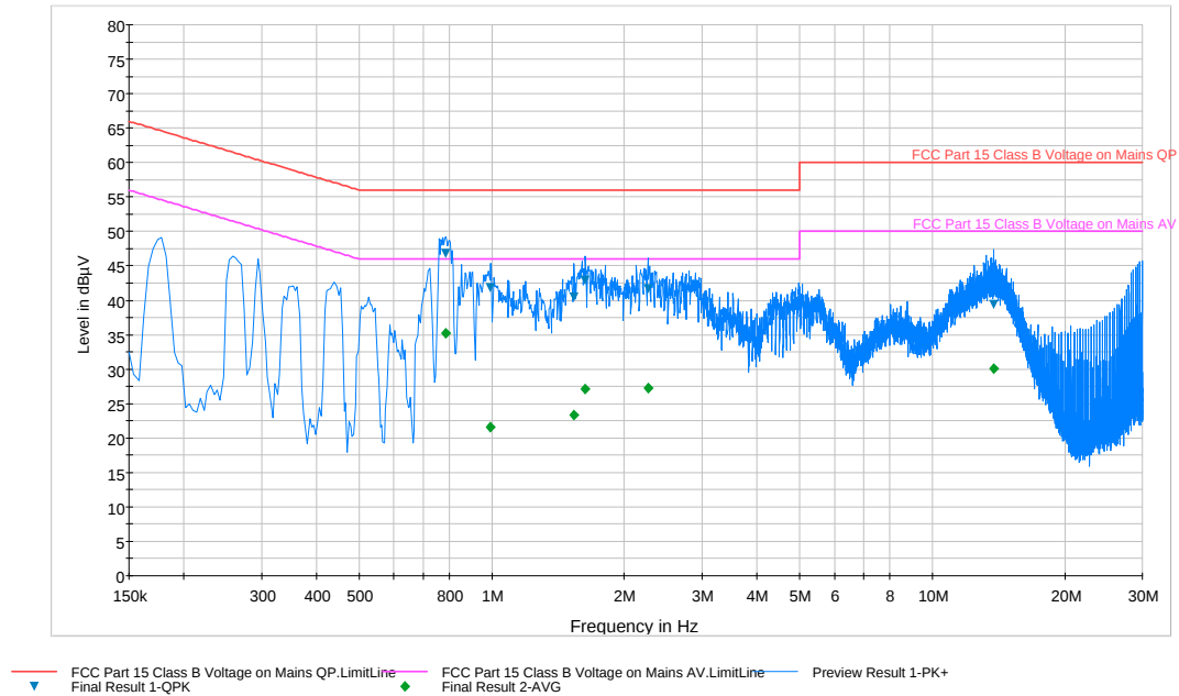
Plot 7-4. Line Conducted Plot (LN) – Battery at 50%
