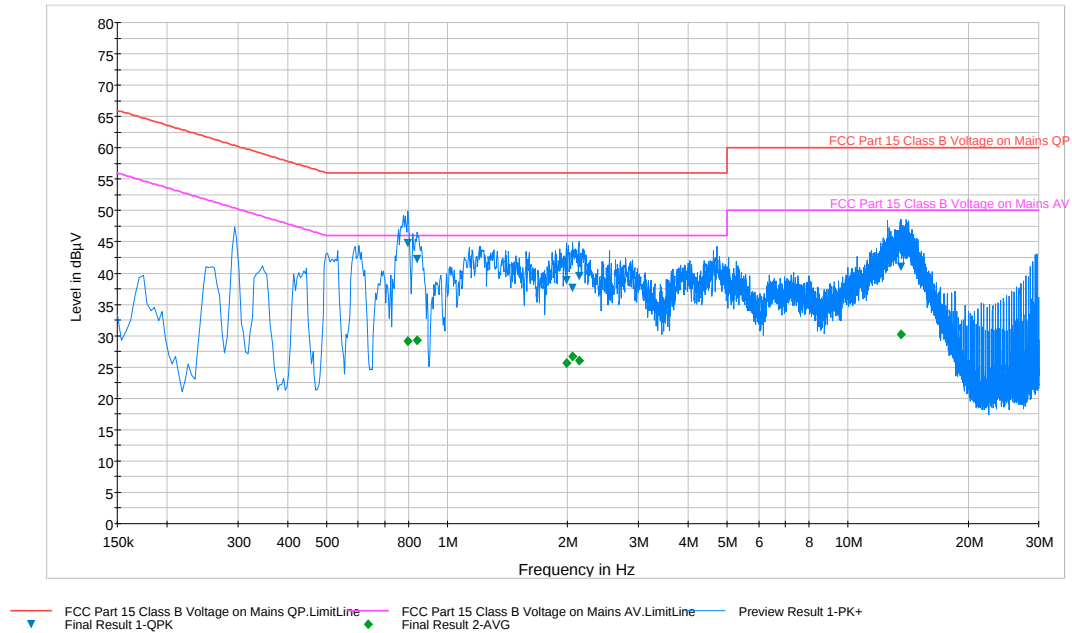
Plot 7-8. Line Conducted Plot (LN) – Max Resistive Load
