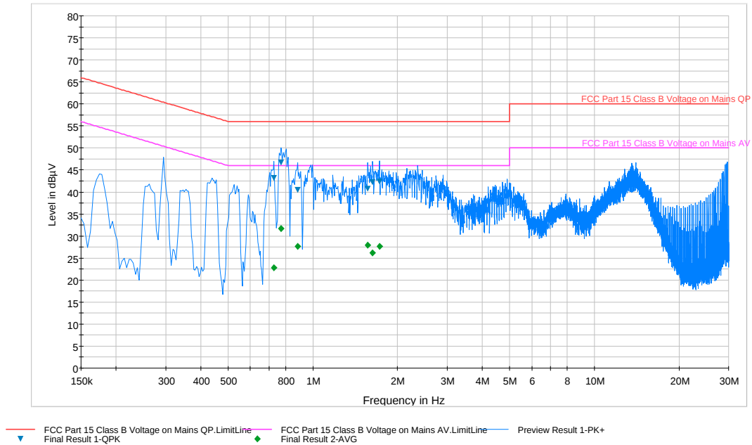
Plot 7-2. Line Conducted Plot (LN) – Battery at 0%
