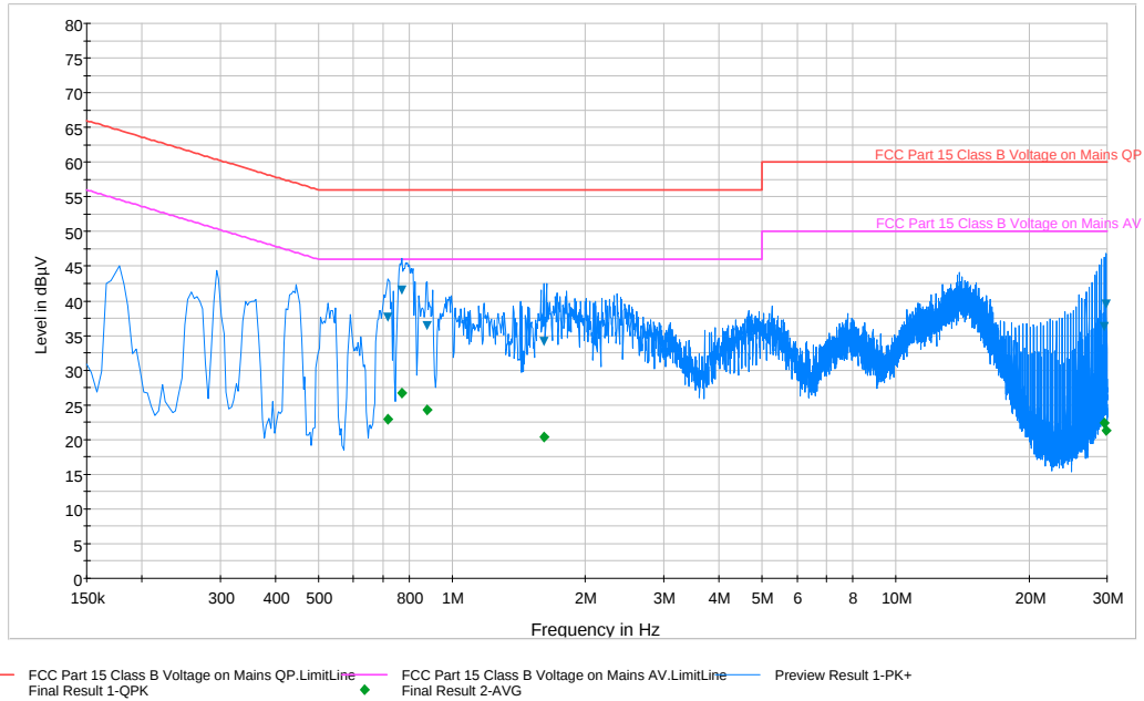
Plot 7-3. Line Conducted Plot (L1) – Battery at 50%
