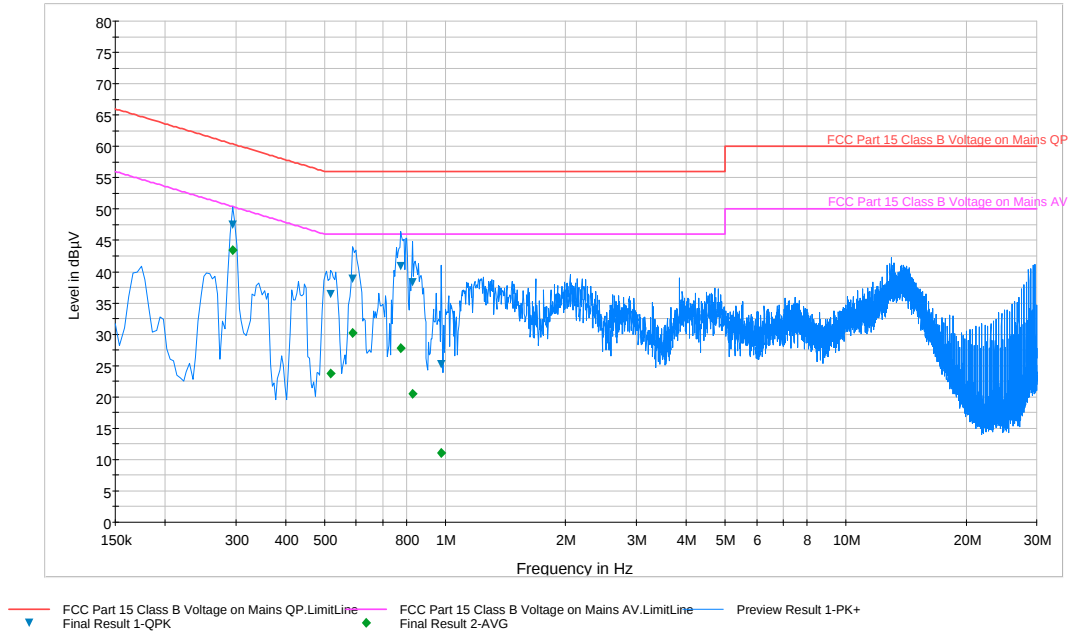
Plot 7-7. Line Conducted Plot (L1) – Max Resistive Load
