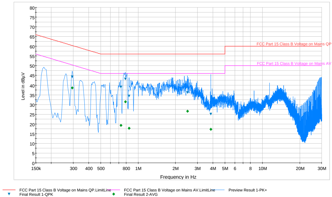
Plot 7-1. Line Conducted Plot (L1) – Battery at 0%
