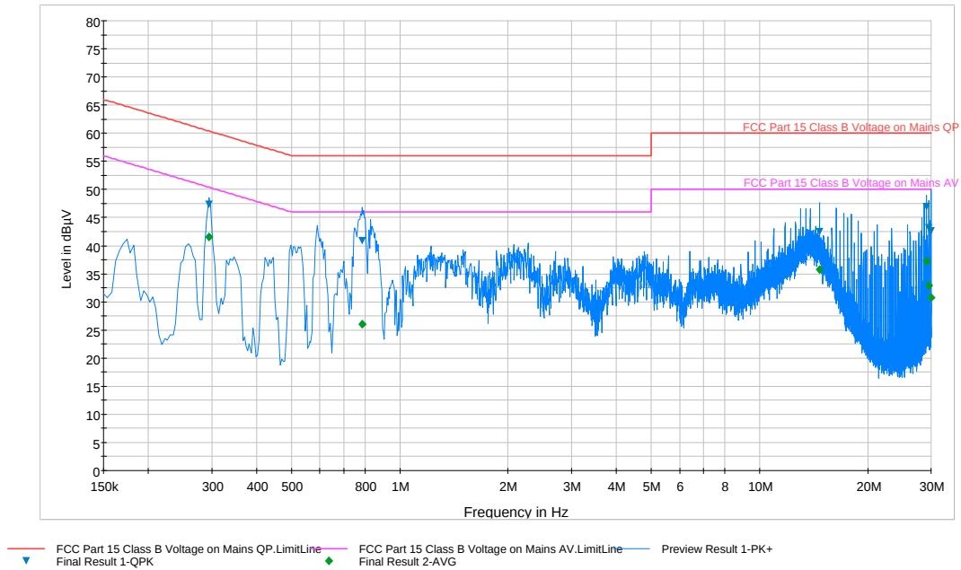
Plot 7-5. Line Conducted Plot (L1) – Battery at 100%
