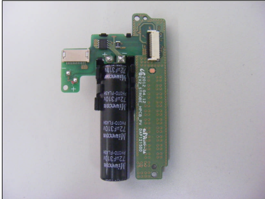
Top view of Strobe PCB
