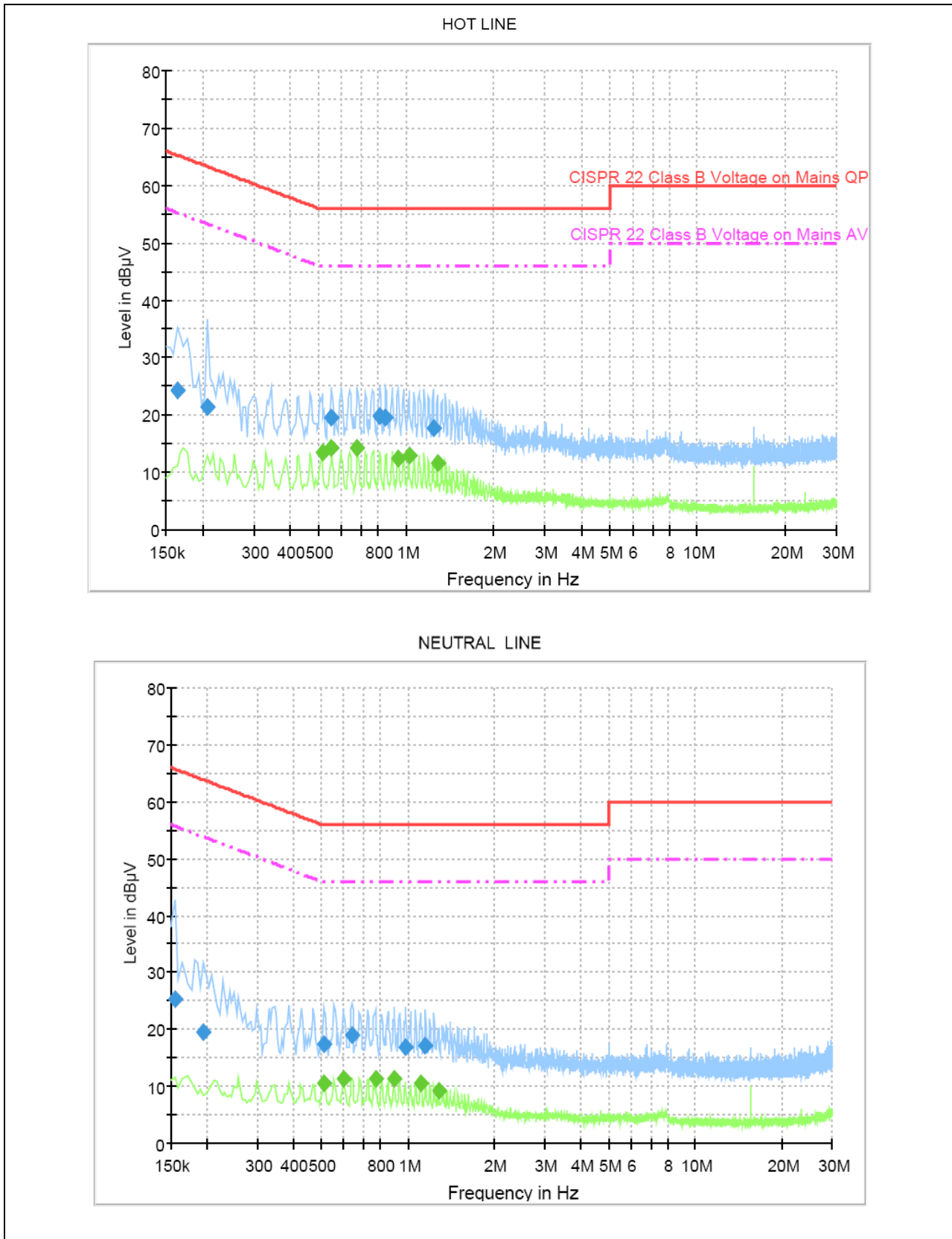
Figure 5. Graphical representation of Conducted Emission
