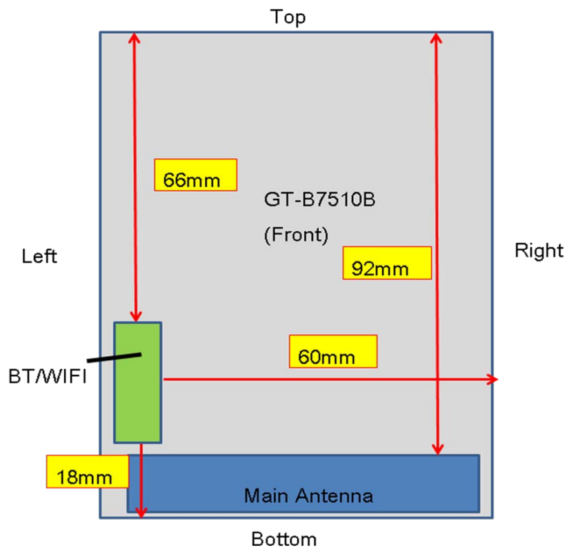
Figure 13-1 Identification of Sides for SAR Testing
