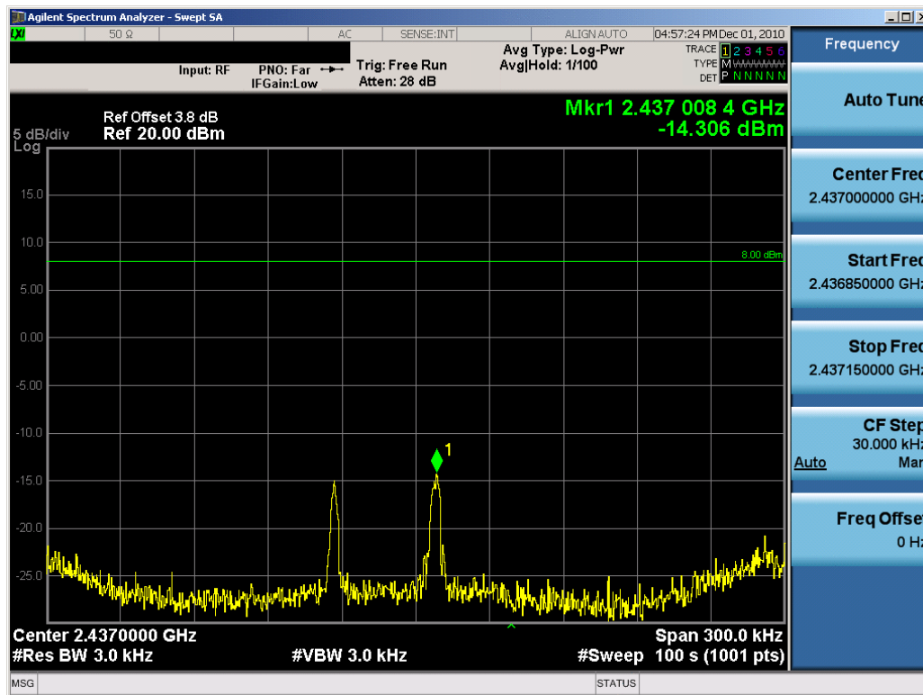
Plot 6-11. Power Spectral Density Plot (802.11g – Ch. 6)
