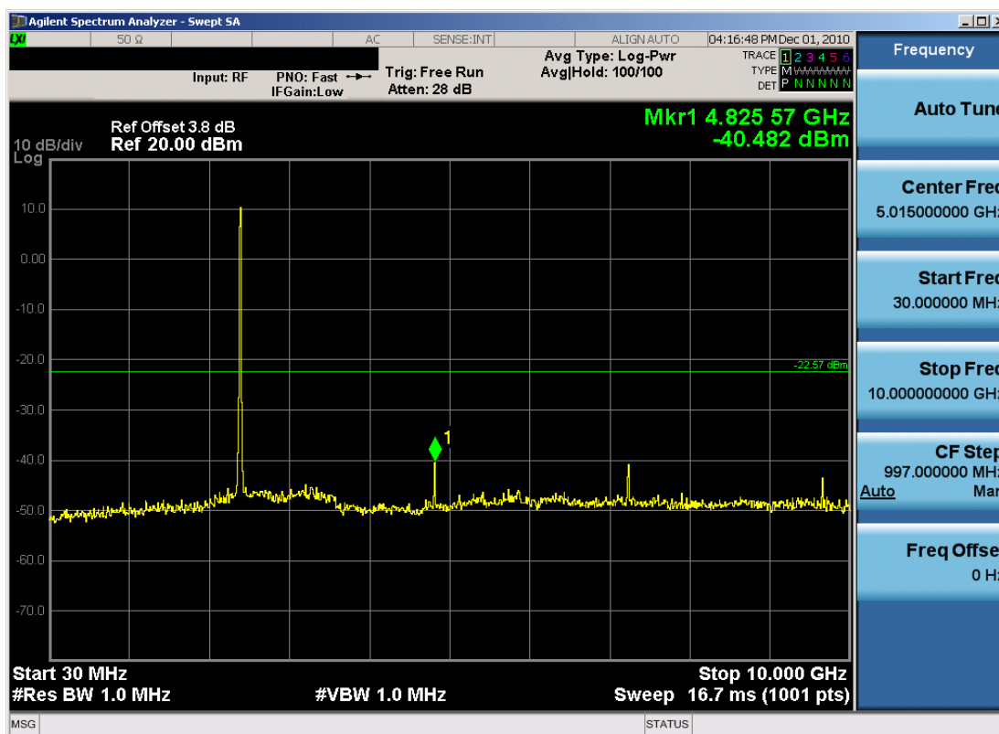
Plot 6-17. Conducted Spurious Plot (802.11b – Ch. 1)
