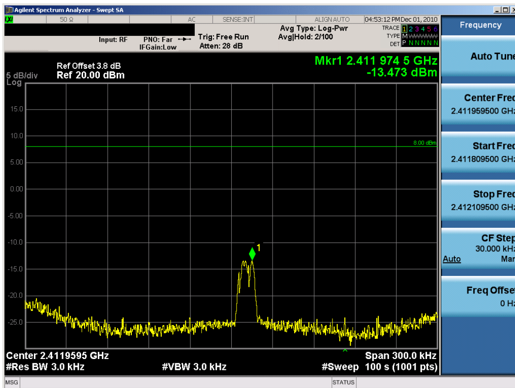
Plot 6-10. Power Spectral Density Plot (802.11g – Ch. 1)
