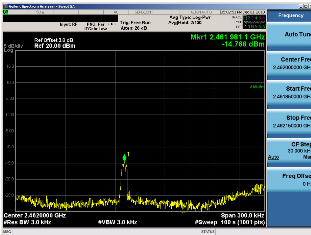
Plot 6-12. Power Spectral Density Plot (802.11g – Ch. 11)
