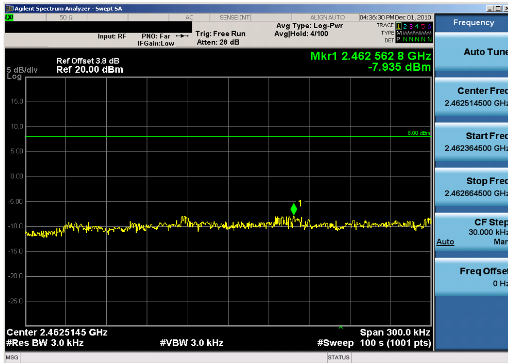
Plot 6-9. Power Spectral Density Plot (802.11b – Ch. 11)
