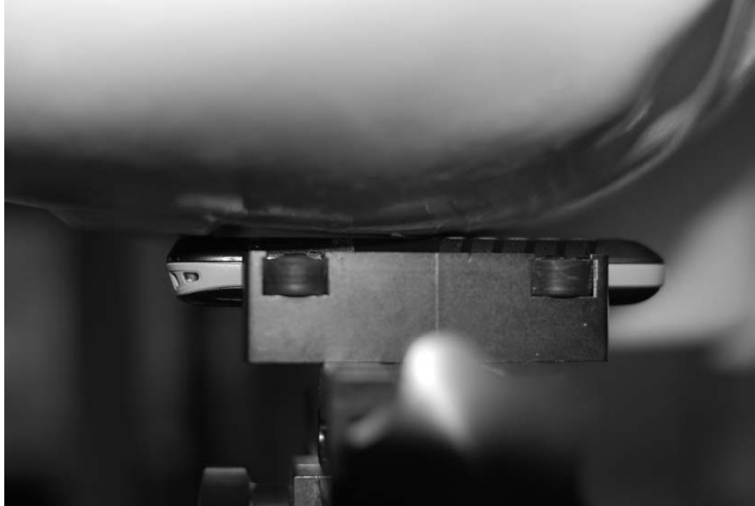
Figure 18-1 SAR Test Setup Photo 1
