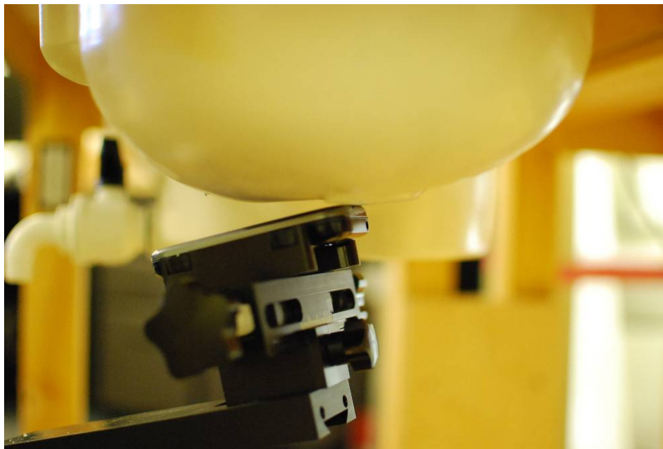
SAR Test Setup Photo 4 – Left Tilt, Slide In
