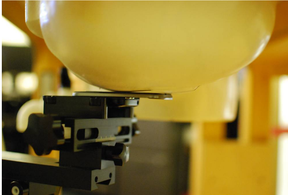
SAR Test Setup Photo 7 – Left Touch, Slide Out
