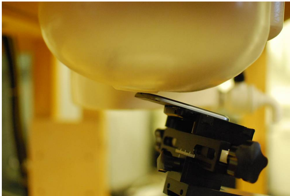
SAR Test Setup Photo 6 – Right Tilt, Slide Out
