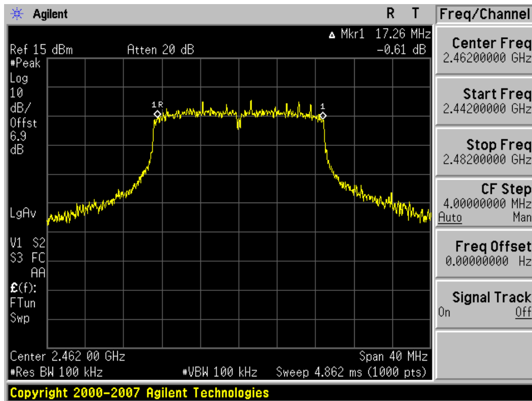
Plot 6-9. 6dB Bandwidth Plot (802.11n – Ch. 11)
