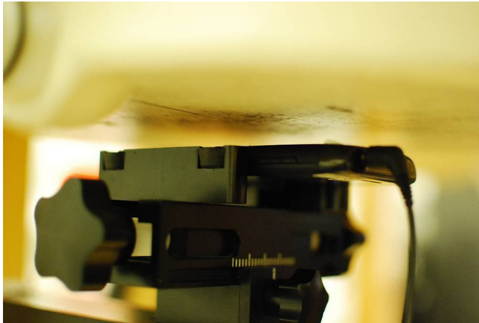
SAR Test Setup Photo 10 – Body-Worn back at 1.0 cm
