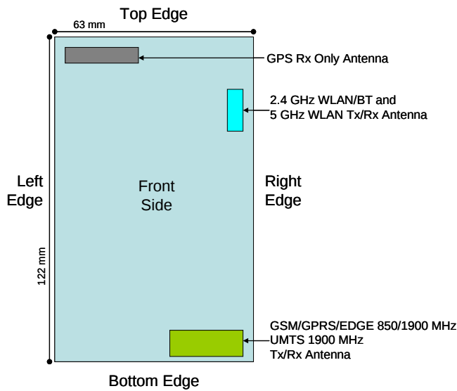
Figure 1-1 DUT Antenna Locations
