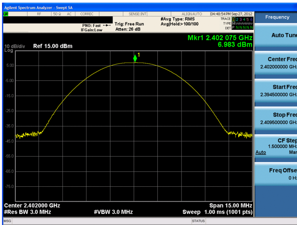
Plot 6-4. Peak Conducted Power (1Mbps – Ch. 0)
