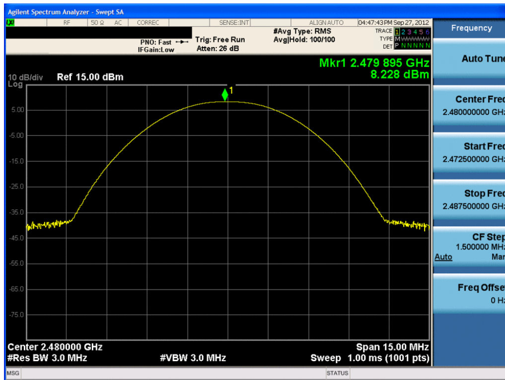
Plot 6-6. Peak Conducted Power (1Mbps – Ch. 78)
