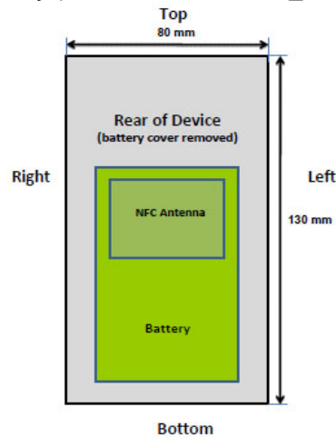
Figure 1-2 NFC Antenna Locations
