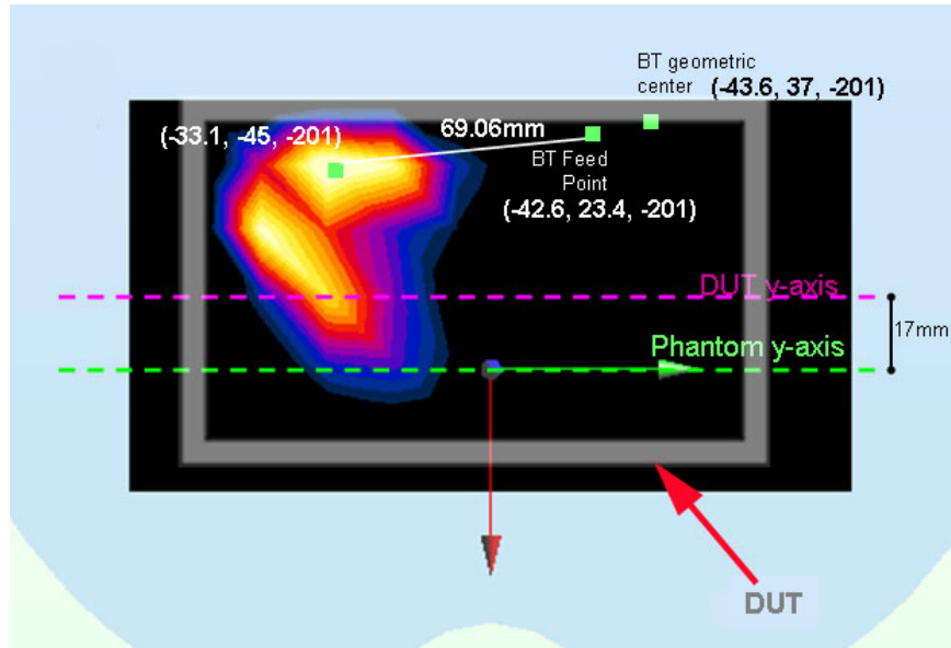
Figure 11-2 Peak SAR Location Plot of UMTS1900 and Bluetooth
