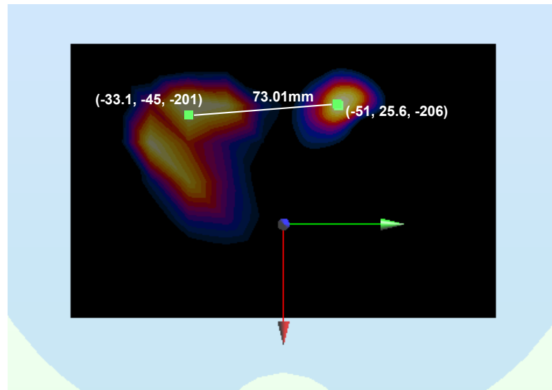
Figure 11-1 Peak SAR Location Plot of UMTS1900 and 2.4 GHz WLAN
