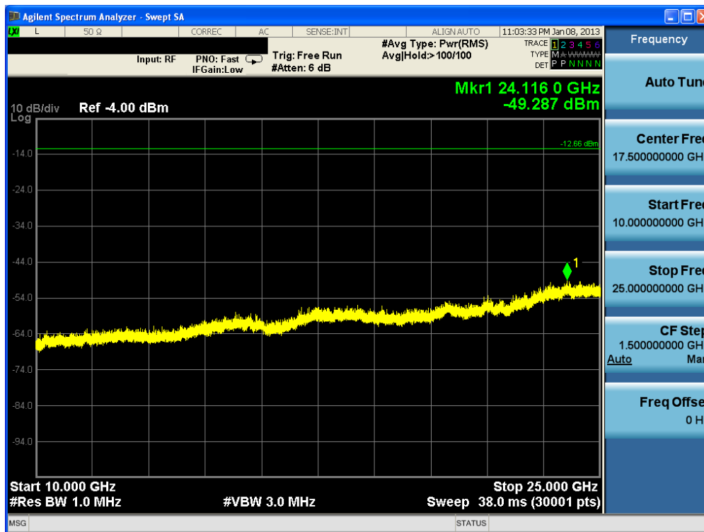
Plot 6-12. Conducted Spurious Plot (Bluetooth (LE) – Ch. 19)
