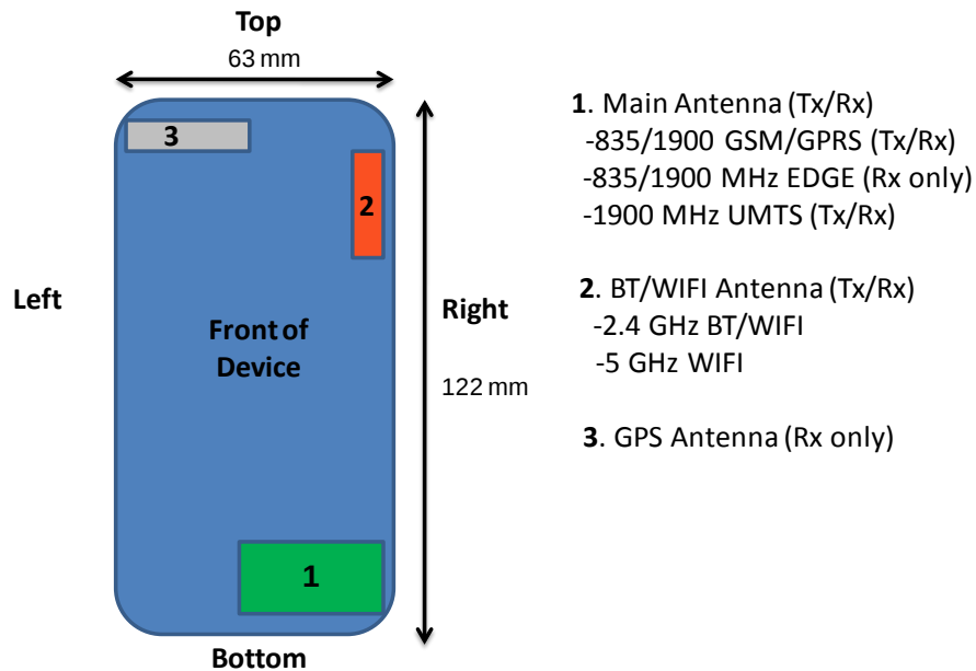
Figure 1-1 DUT Antenna Locations
