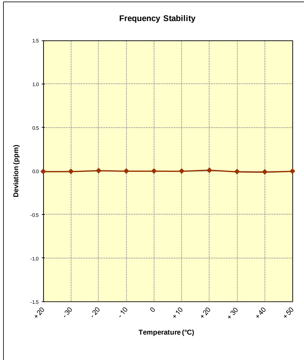
Figure 6-9. Frequency Stability Graph (PCS WCDMA Mode – Ch. 9400)
