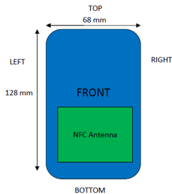
Figure 1-2 NFC Antenna Locations
