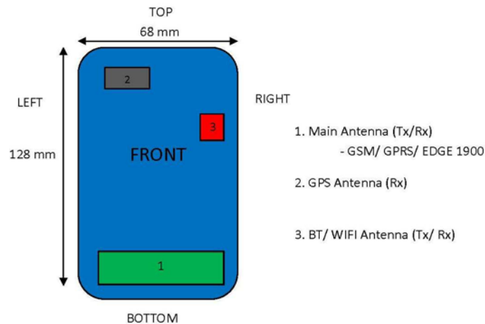
Figure 1-1 DUT Antenna Locations
