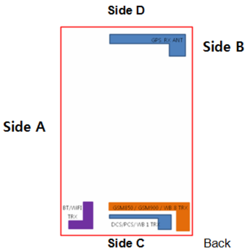
Figure 5.7 Identification of Sides for SAR Testing
