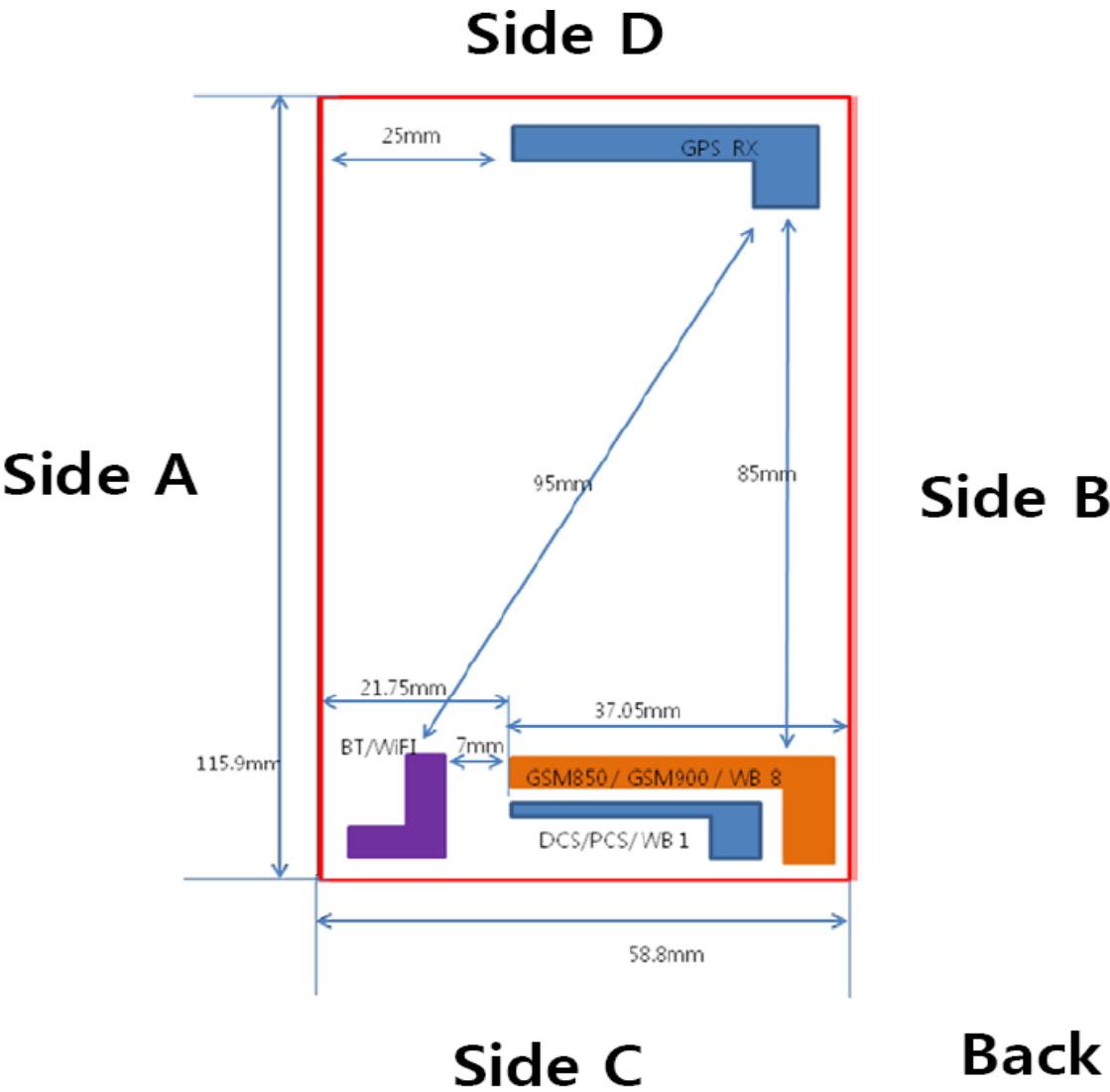
Figure 5.8 Antenna Locations, as viewed from back of device
