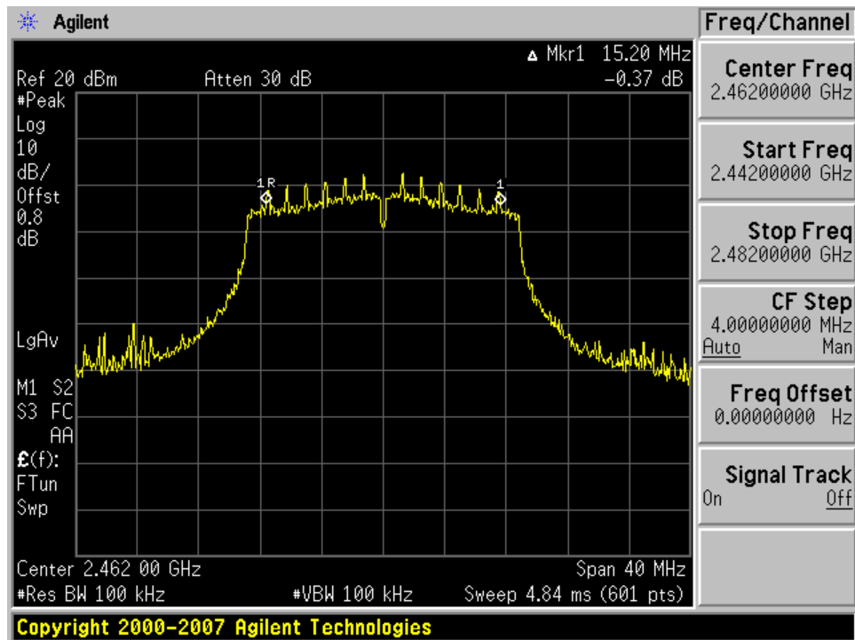
Plot 6-9. 6dB Bandwidth Plot (802.11n – Ch. 11)
