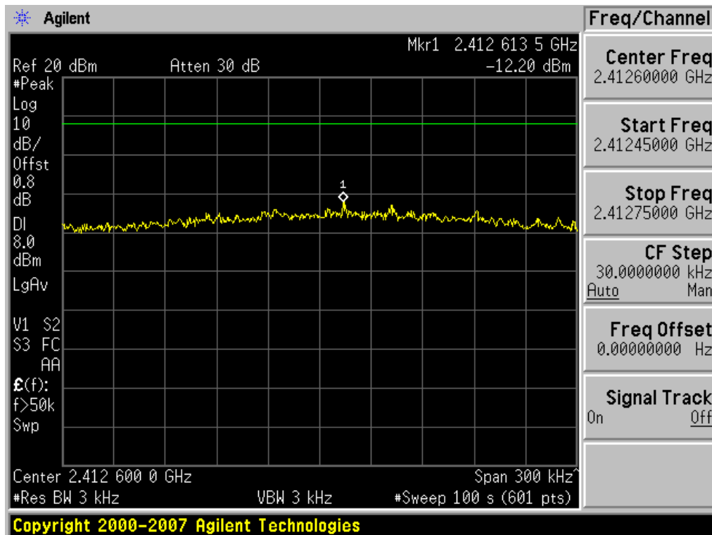
Plot 6-16. Power Spectral Density Plot (802.11n – Ch. 1)
