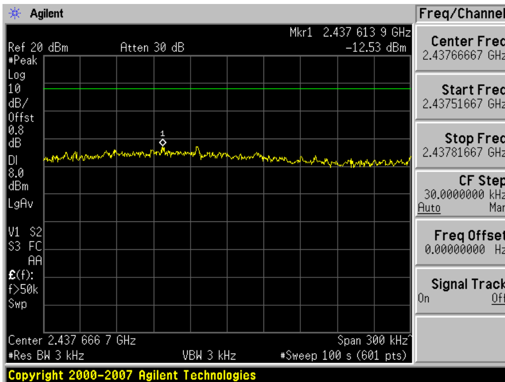
Plot 6-17. Power Spectral Density Plot (802.11n – Ch. 6)
