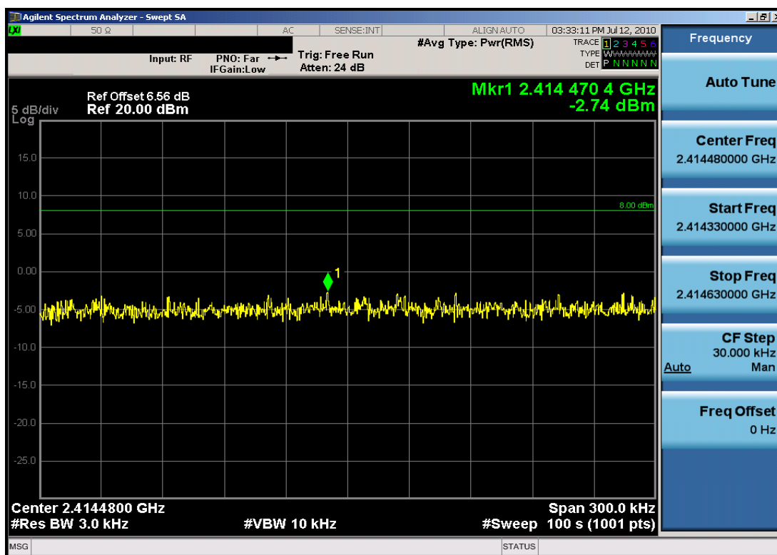
Plot 6-4. Power Spectral Density Plot (802.11b – Ch. 1)
