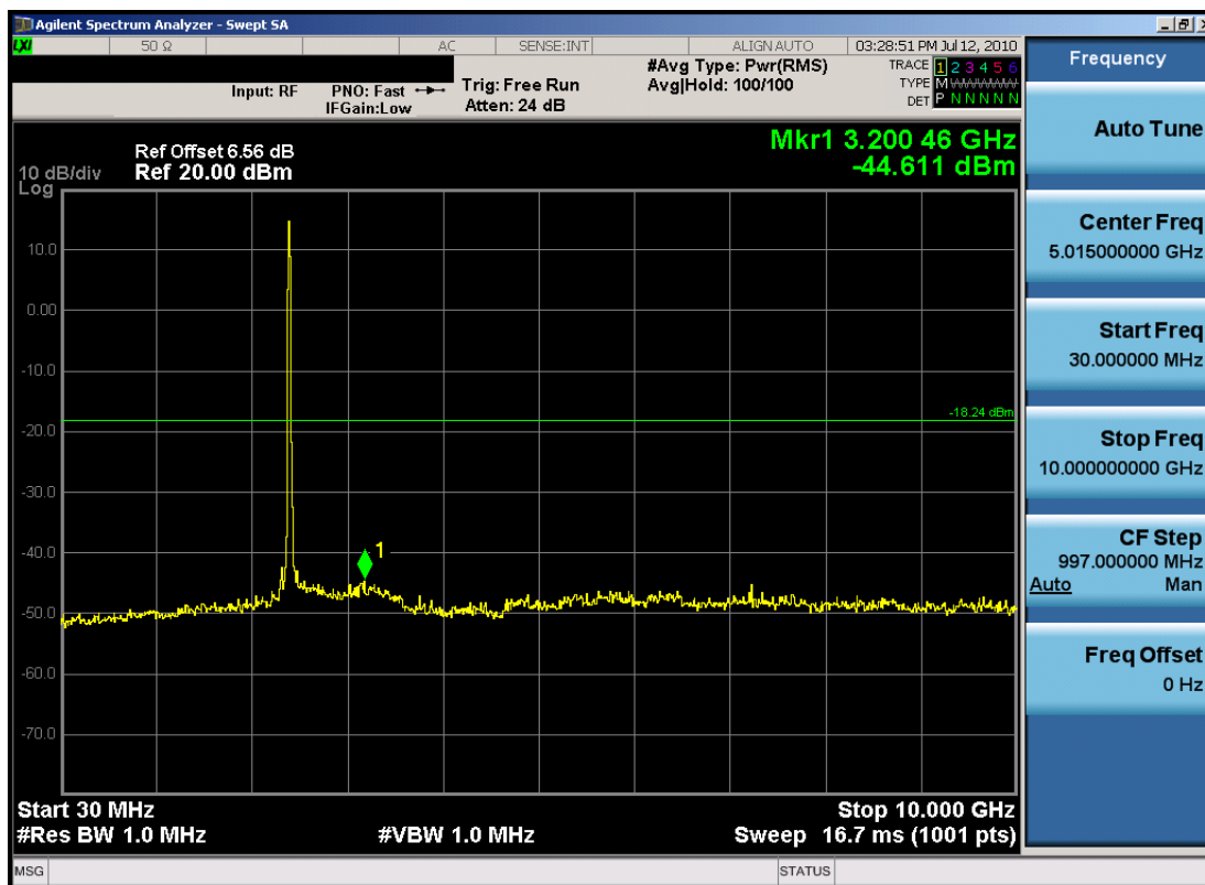
Plot 6-13. Conducted Spurious Plot (802.11b – Ch. 1)
