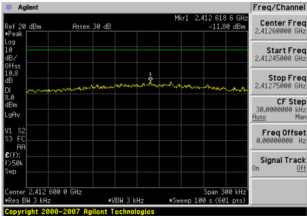
Plot 6-16. Power Spectral Density Plot (802.11n - Ch. 1)
