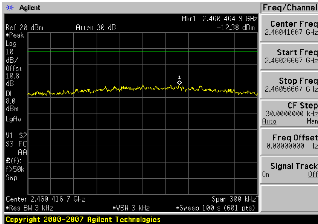
Plot 6-18. Power Spectral Density Plot (802.11n – Ch. 11)
