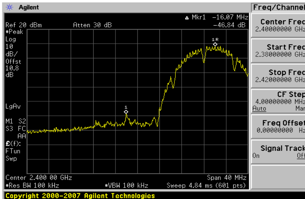
Plot 6-19. Band Edge Plot (802.11b – Ch. 1)
