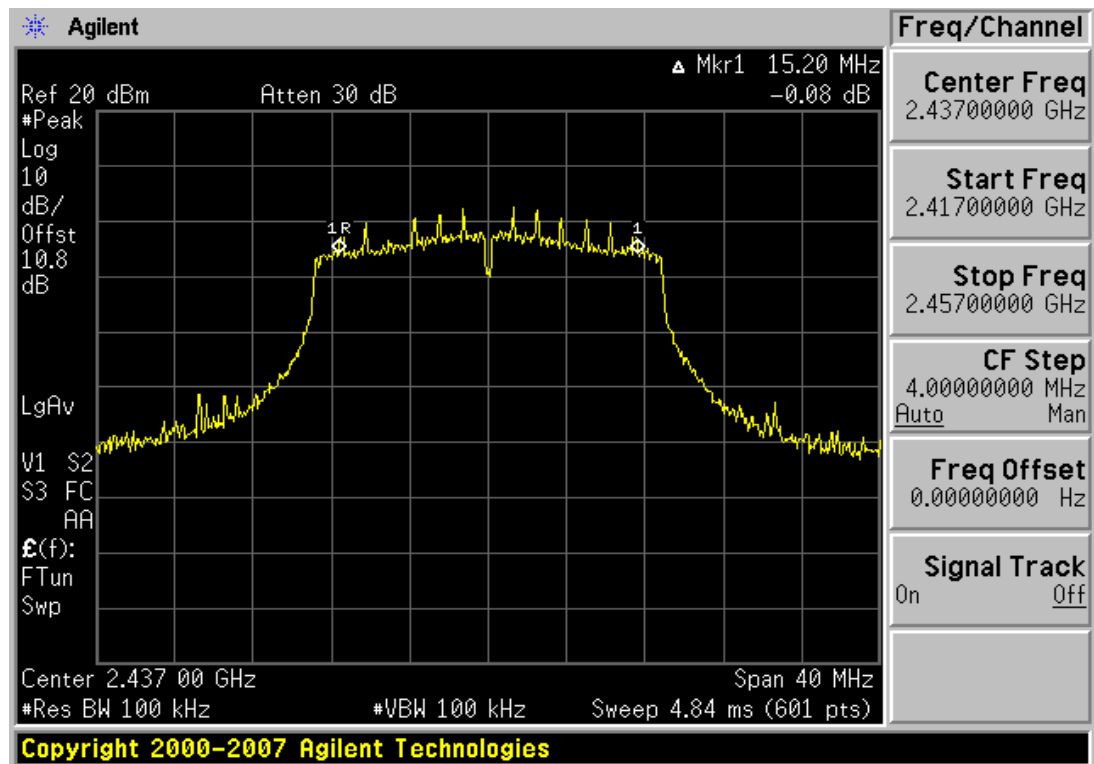
Plot 6-8. 6dB Bandwidth Plot (802.11n - Ch. 6)
