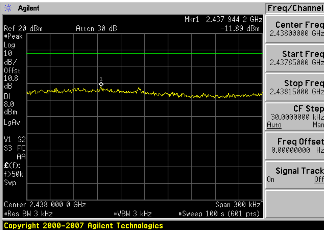
Plot 6-17. Power Spectral Density Plot (802.11n - Ch. 6)
