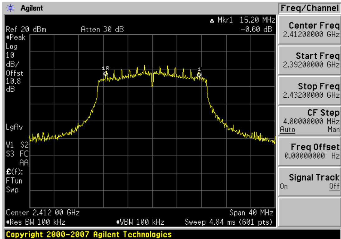
Plot 6-7. 6dB Bandwidth Plot (802.11n - Ch. 1)
