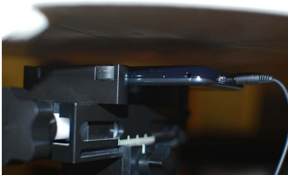
Figure 19-5 SAR Test Setup Photo 5
