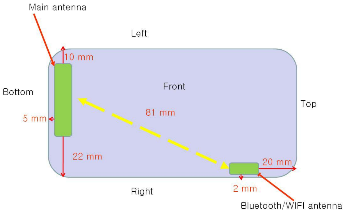
Figure 13-1 Identification of Sides for SAR Testing
