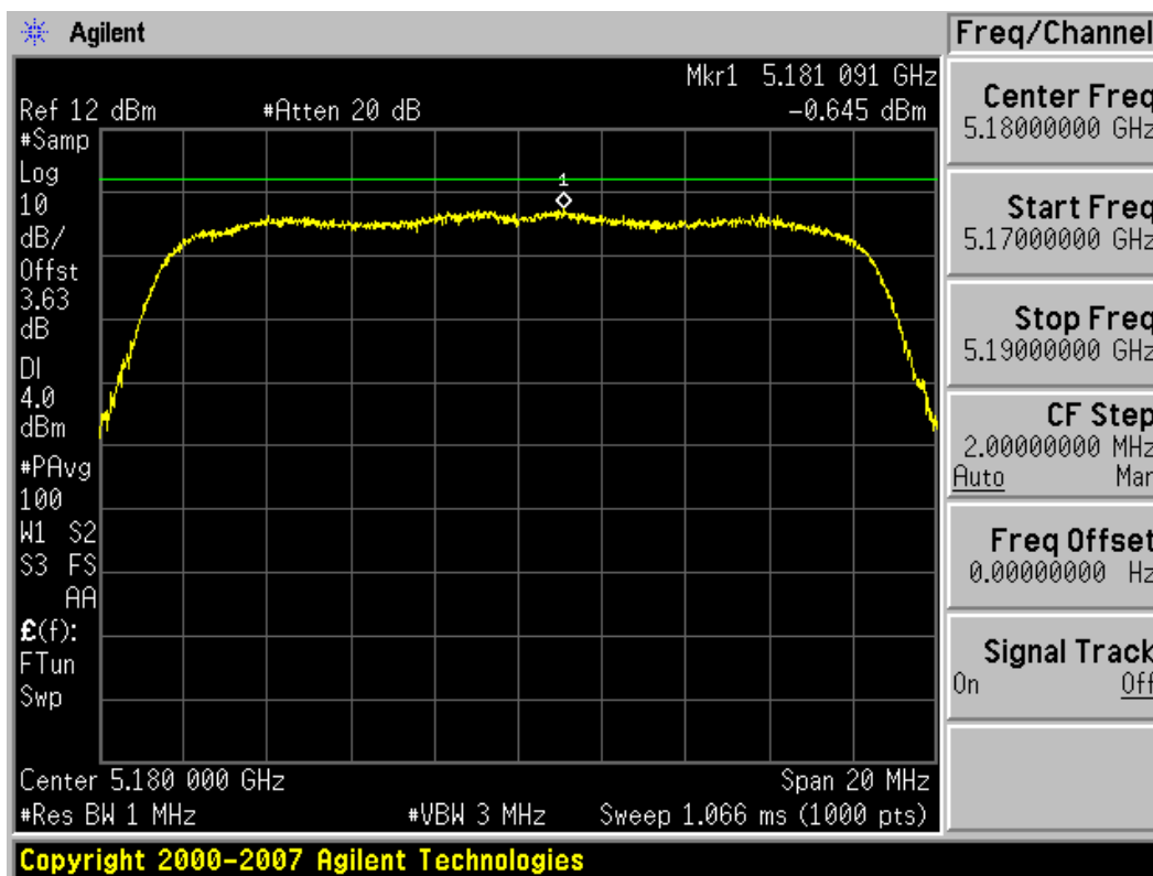
Plot 6-19. Peak Power Spectral Density Plot (802.11a (UNII Band 1) – Ch. 36)
