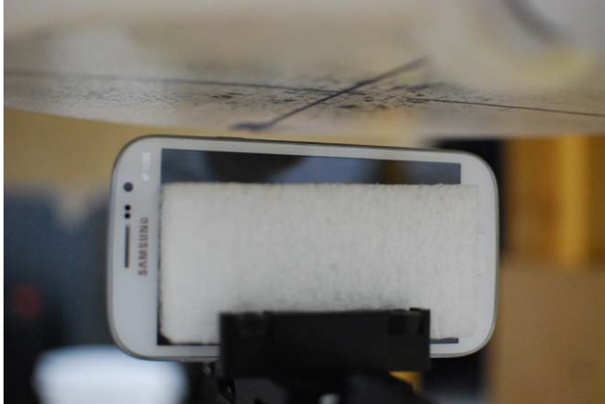
SAR Test Setup Photo 7: Right Edge at 1.0 cm
