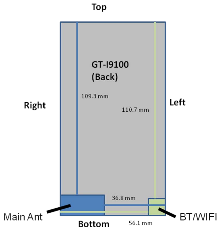
Figure 13-1 Identification of Sides for SAR Testing
