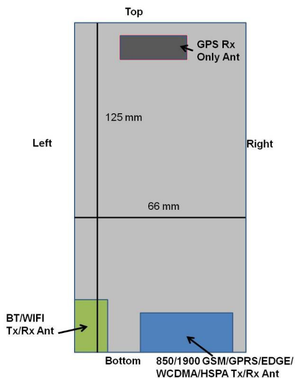
Figure 13-1 Identification of Sides for SAR Testing (Front View)
