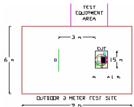
Figure 3-6. Dimensions of Outdoor Test Site
