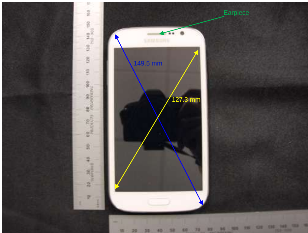
Overall Dimensions
