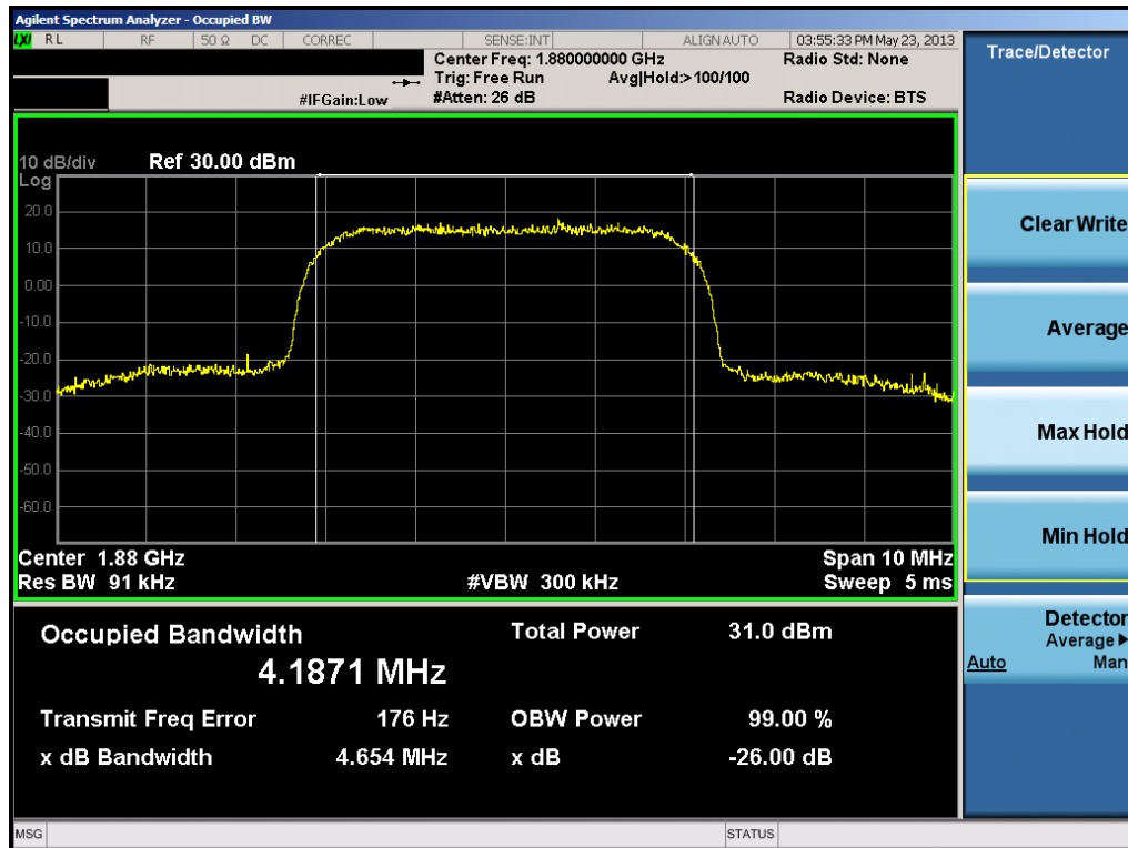
Plot 7-41. Occupied Bandwidth Plot (PCS WCDMA Mode – Ch. 9400)
