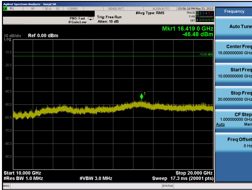
Plot 7-40. Conducted Spurious Plot (PCS WCDMA Mode – Ch. 9400)
