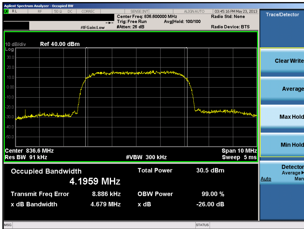
Plot 7-31. Occupied Bandwidth Plot (Cellular WCDMA Mode – Ch. 4183)
