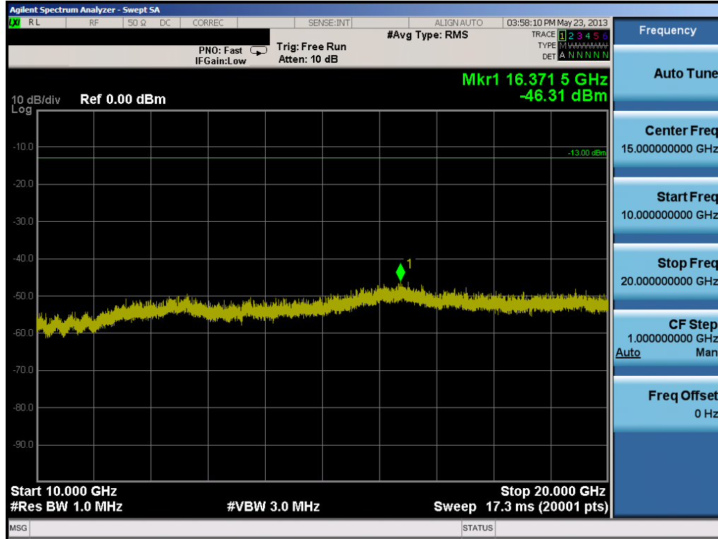
Plot 7-44. Conducted Spurious Plot (PCS WCDMA Mode – Ch. 9538)
