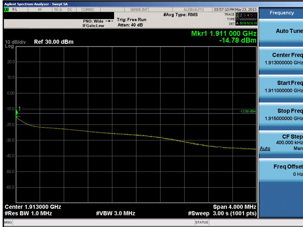
Plot 7-46. 4MHz Span Plot (PCS WCDMA Mode – Ch. 9538)
