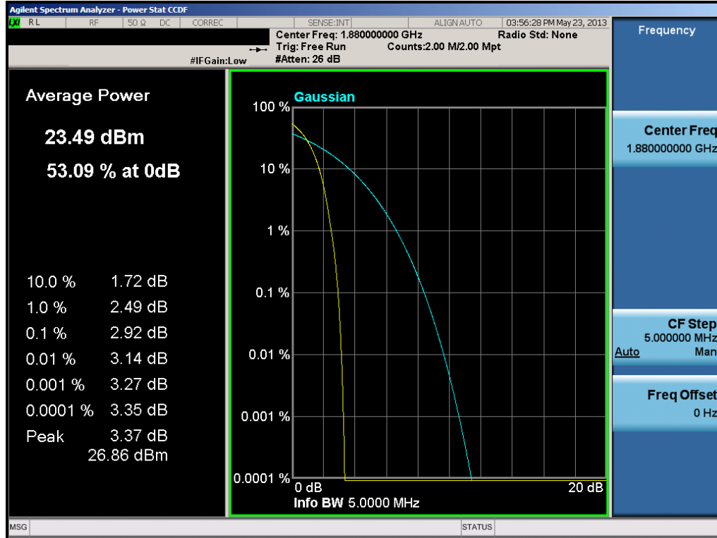
Plot 7-42. Peak-Average Ratio Plot (PCS WCDMA Mode – Ch. 9400)
