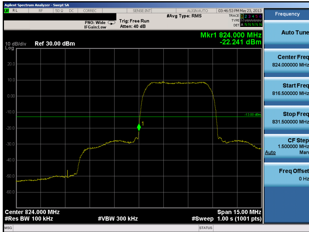
Plot 7-28. Band Edge Plot (Cellular WCDMA Mode – Ch. 4132)
