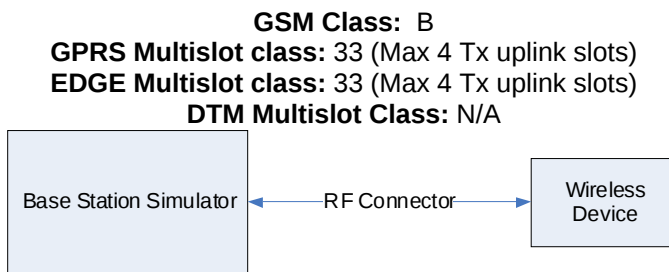
Figure 9-1 Power Measurement Setup
