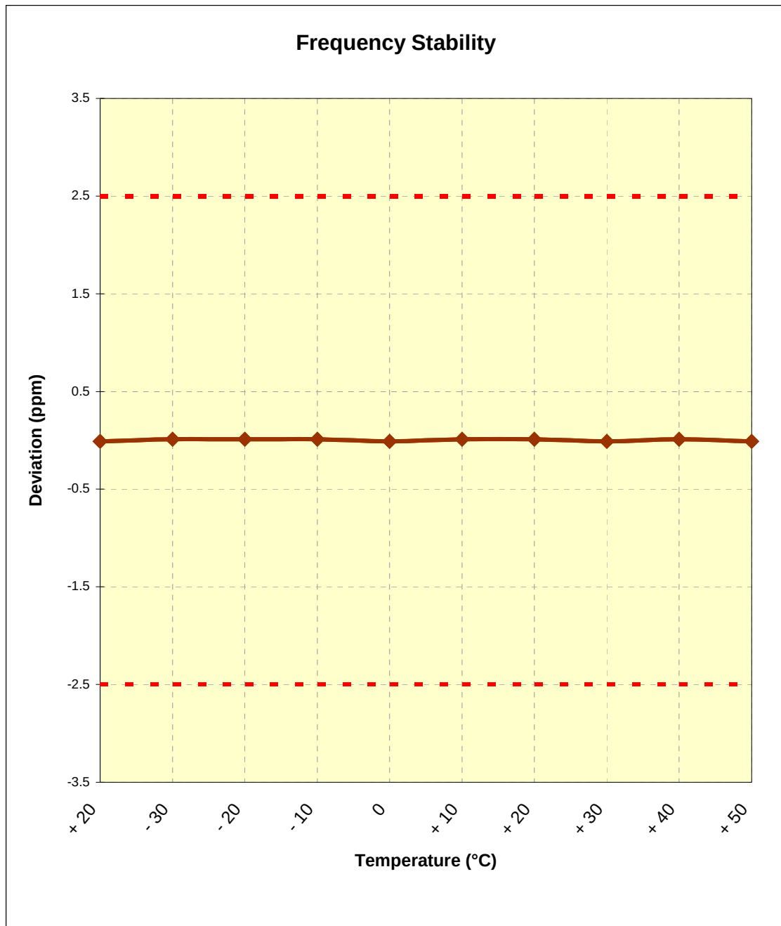
Plot 6-1. Frequency Stability Graph (PCS GSM Mode – Ch. 661)
