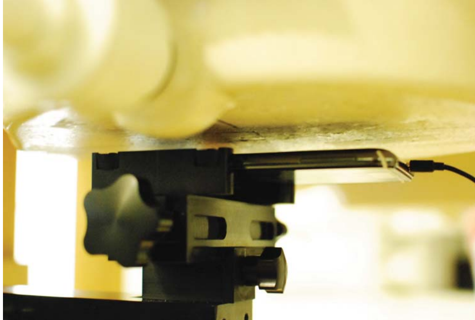
SAR Test Setup Photo 9: Body Worn at 1.0 cm
