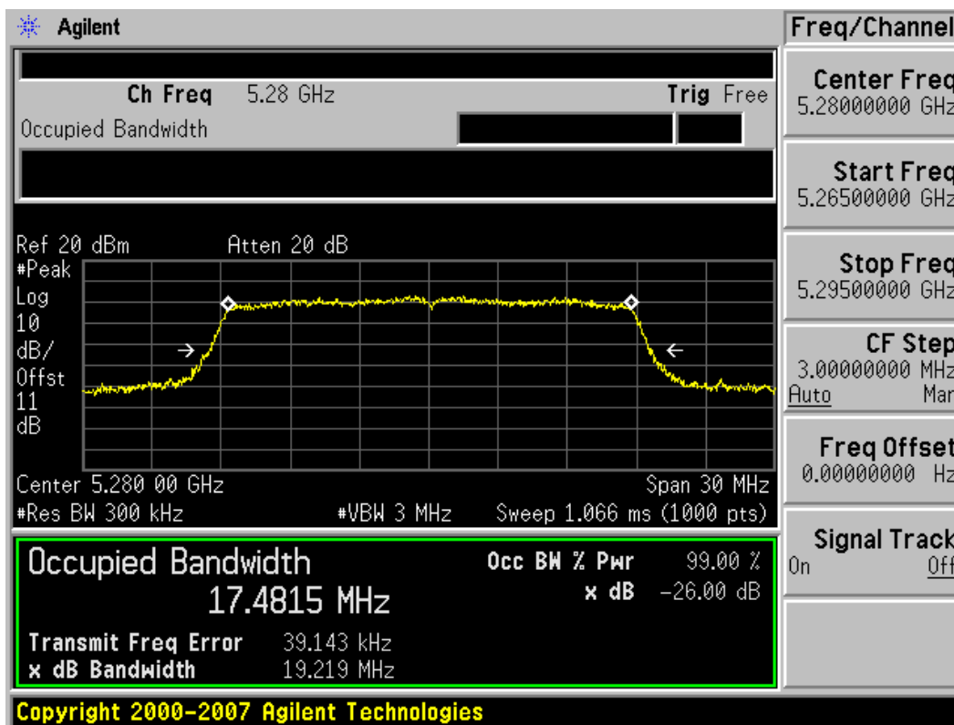
Plot 6-11. 26dB Bandwidth Plot (802.11n (UNII Band 2) – Ch. 56)
