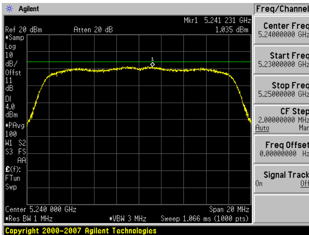
Plot 6-21. Peak Power Spectral Density Plot (802.11a (UNII Band 1) – Ch. 48)
