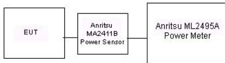
Figure 9-3 Power Measurement Setup for Bandwidths < 50 MHz
