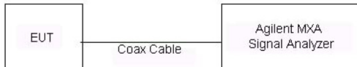
Figure 9-4 Power Measurement Setup for Bandwidths > 50 MHz
