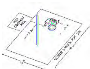
Figure 3-7. Turntable and System Setup
