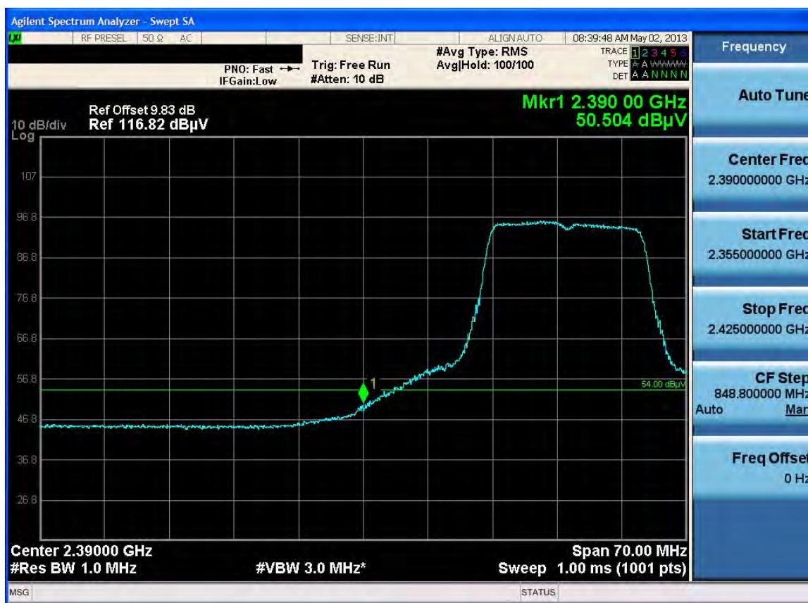
Plot 6-63. Radiated Restricted Lower Band Edge Measurement (Average)
