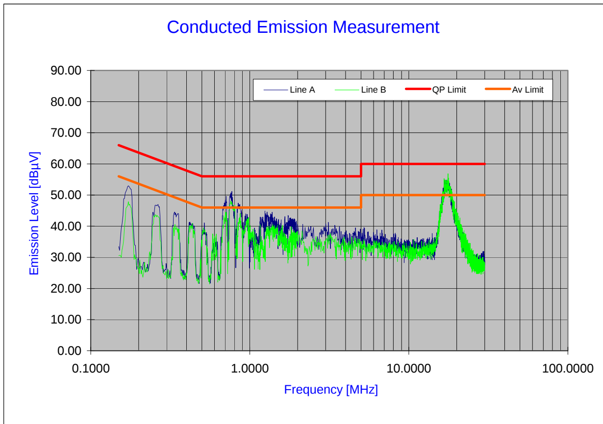
Plot 6-67. Line Conducted Plot with 802.11a
