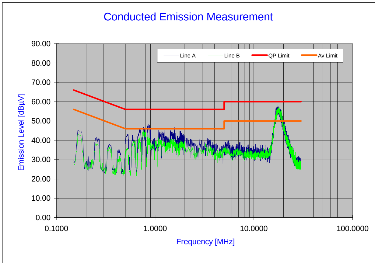
Plot 6-68. Line Conducted Plot with 802.11b
