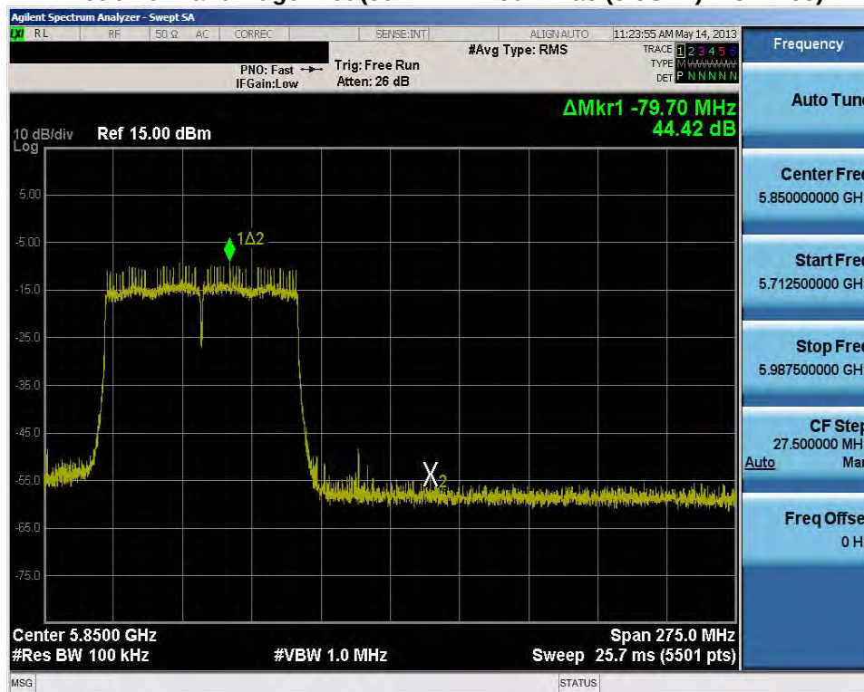
Plot 6-50. Band Edge Plot (80MHz BW 802.11ac (5.8GHz) – Ch. 155)
