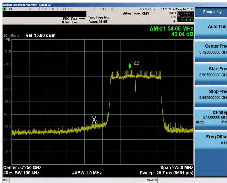
Plot 6-49. Band Edge Plot (80MHz BW 802.11ac (5.8GHz) – Ch. 155)
