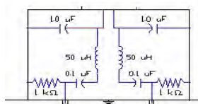
Figure 3-4. LISN Schematic Diagram
