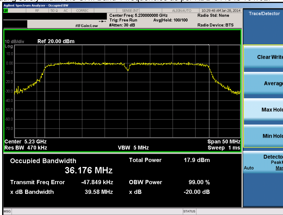
Plot 6-28. 20dB Bandwidth Plot (40MHz 802.11n (UNII Band 1) – Ch. 46)
