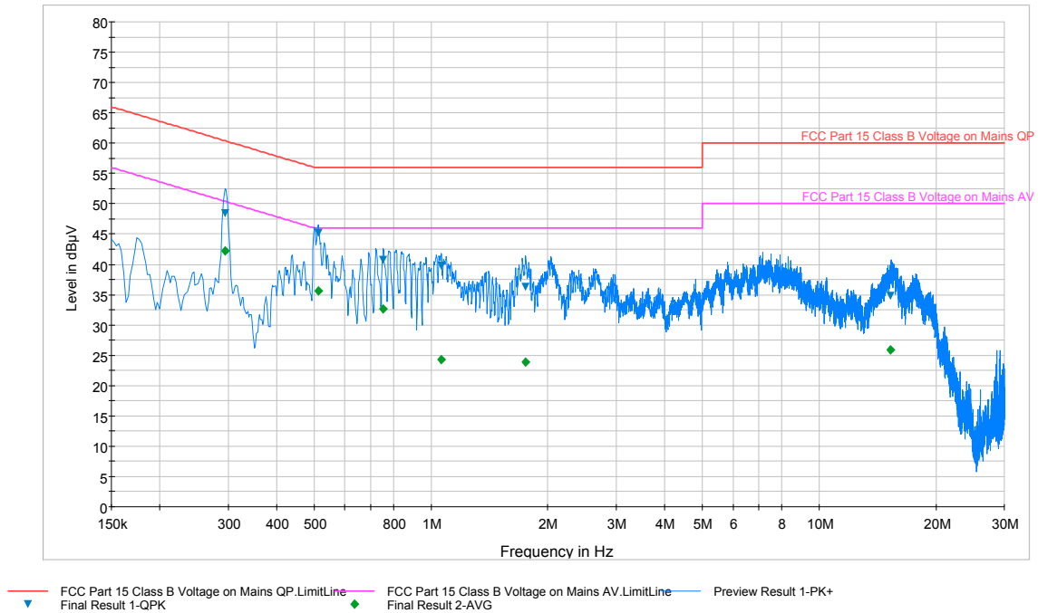
Plot 6-72. Line Conducted Plot with 802.11a UNII Band 1 (L1)
