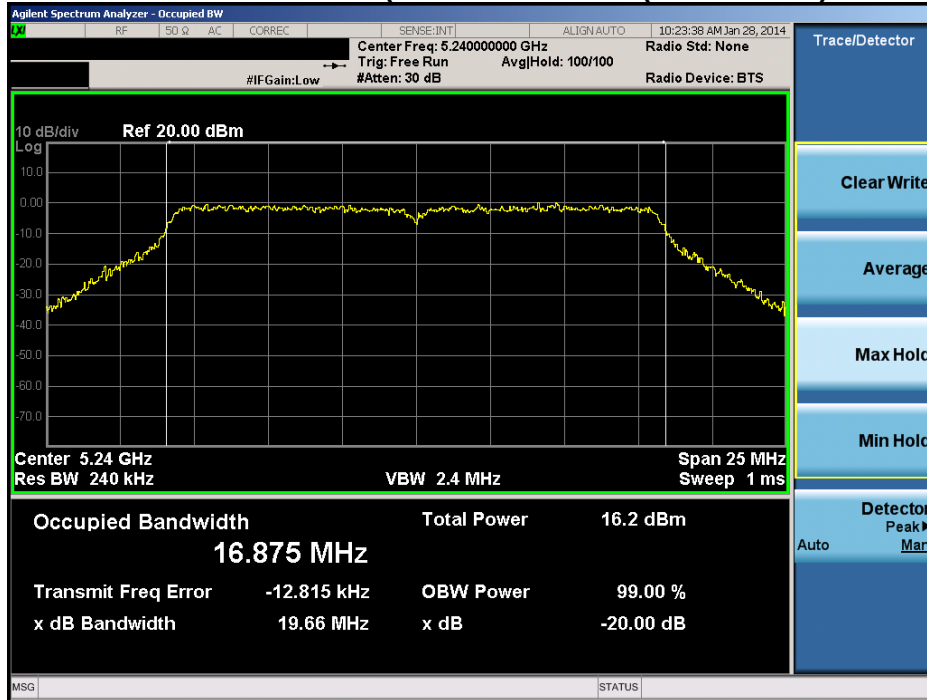
Plot 6-26. 20dB Bandwidth Plot (20MHz 802.11a (UNII Band 1) – Ch. 48)
