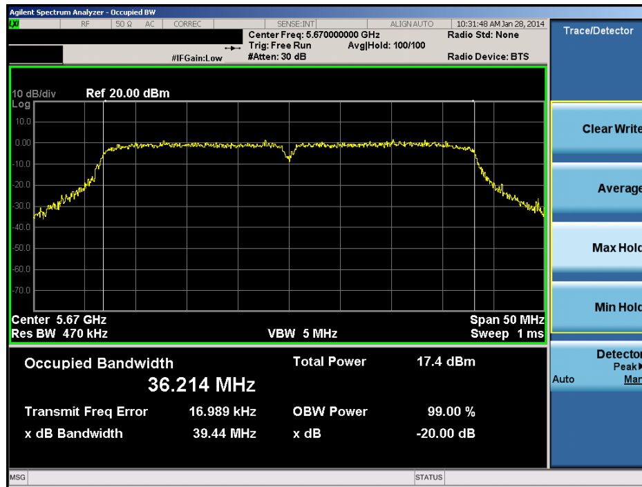
Plot 6-29. 20dB Bandwidth Plot (40MHz 802.11n (UNII Band 2C) – Ch 134)
