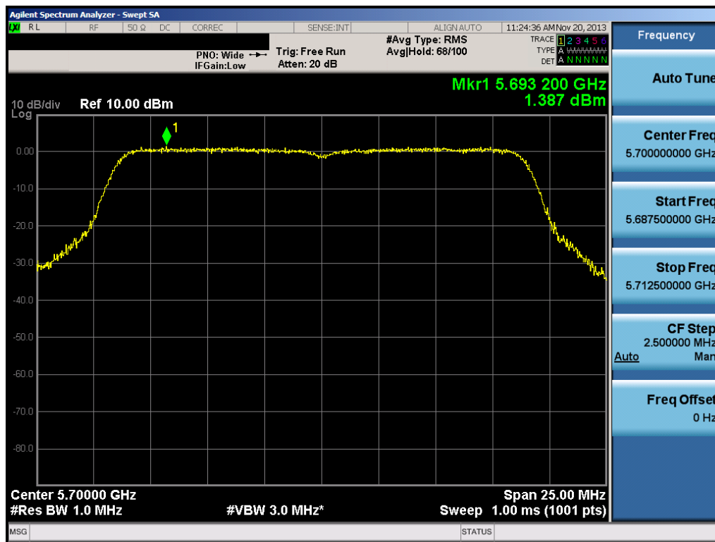
Plot 6-51. Peak Power Spectral Density Plot (20MHz BW 802.11n (UNII Band 2C) – Ch. 140)
