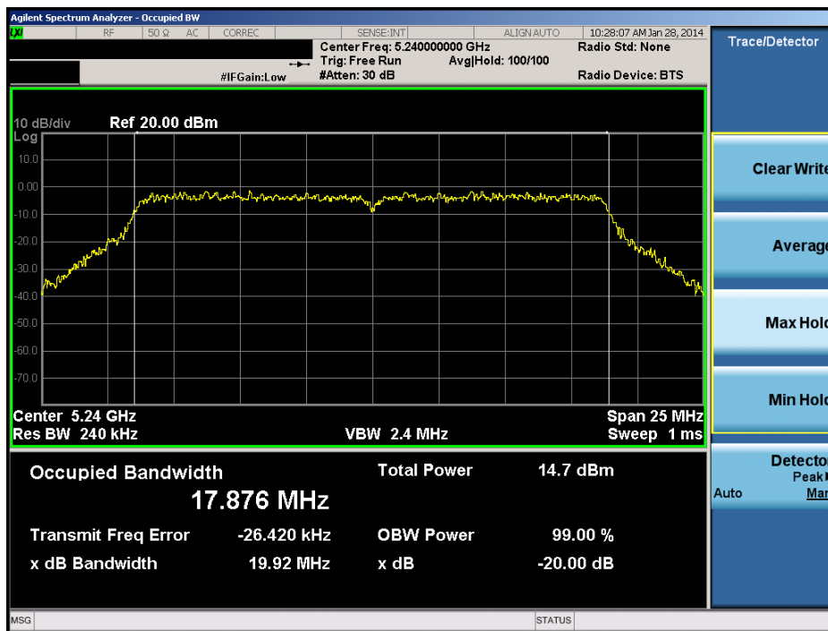
Plot 6-27. 20dB Bandwidth Plot (20MHz 802.11n (UNII Band 1) – Ch. 48)
