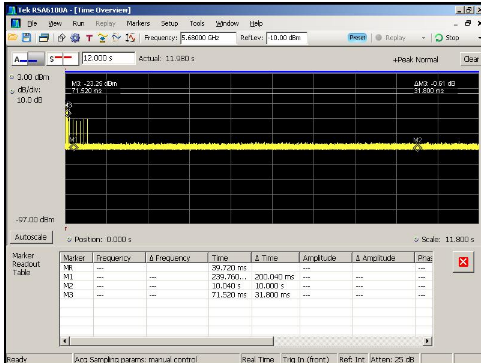
Figure 6-4. Channel Move Time
