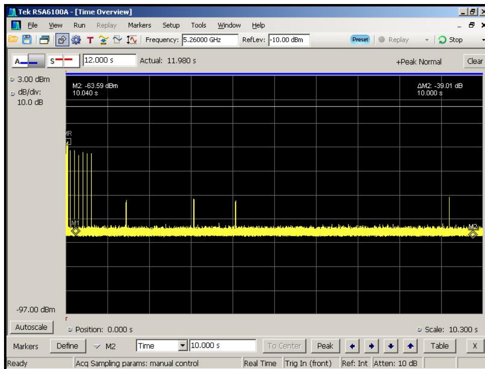
Figure 5-4. Channel Move Time (< 10sec)
