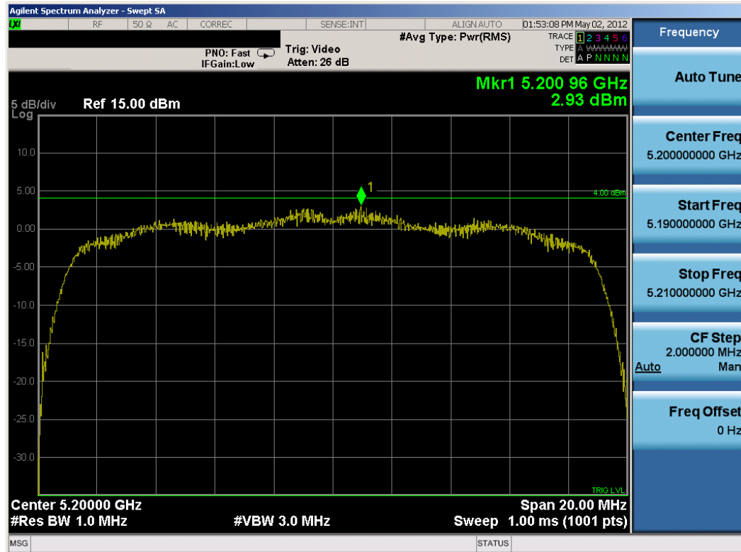
Plot 6-30. Peak Power Spectral Density Plot (20MHz 802.11n (UNII Band 1) – Ch. 40)
