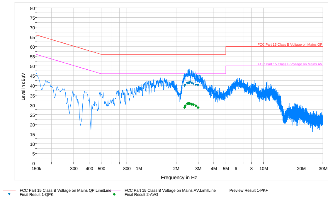
Plot 6-77. Line Conducted Plot with 802.11a (UNII Band 1) (LN)
