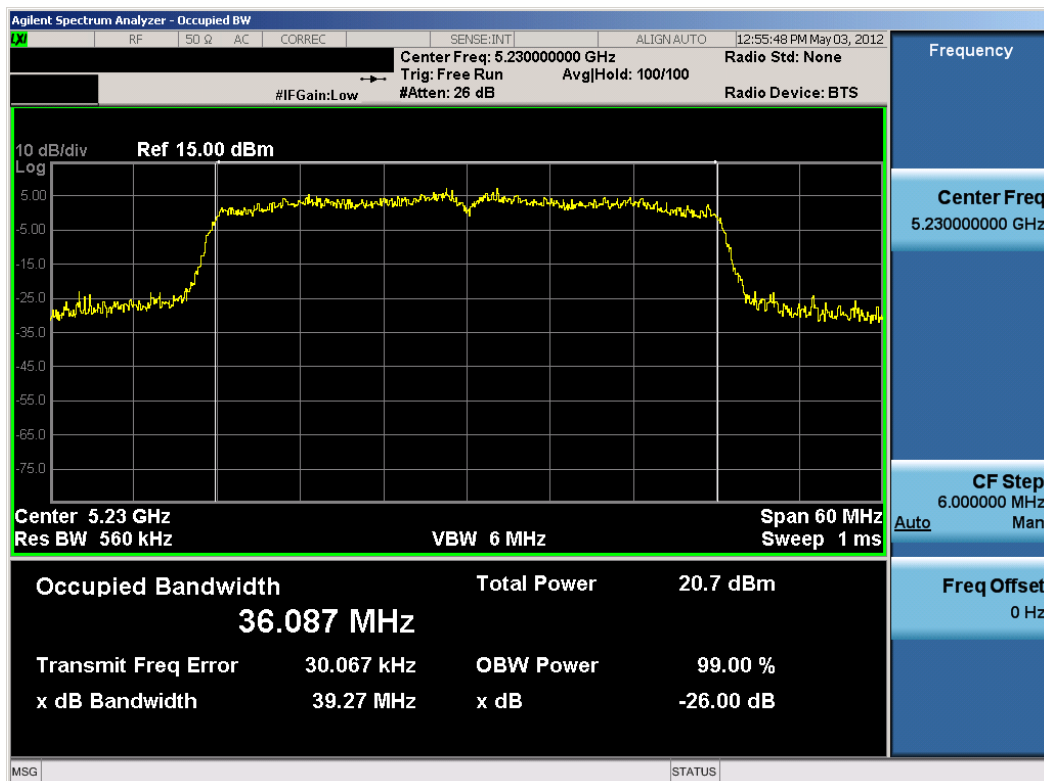
Plot 6-20. 26dB Bandwidth Plot (40MHz 802.11a/n (UNII Band 1) – Ch. 46)
