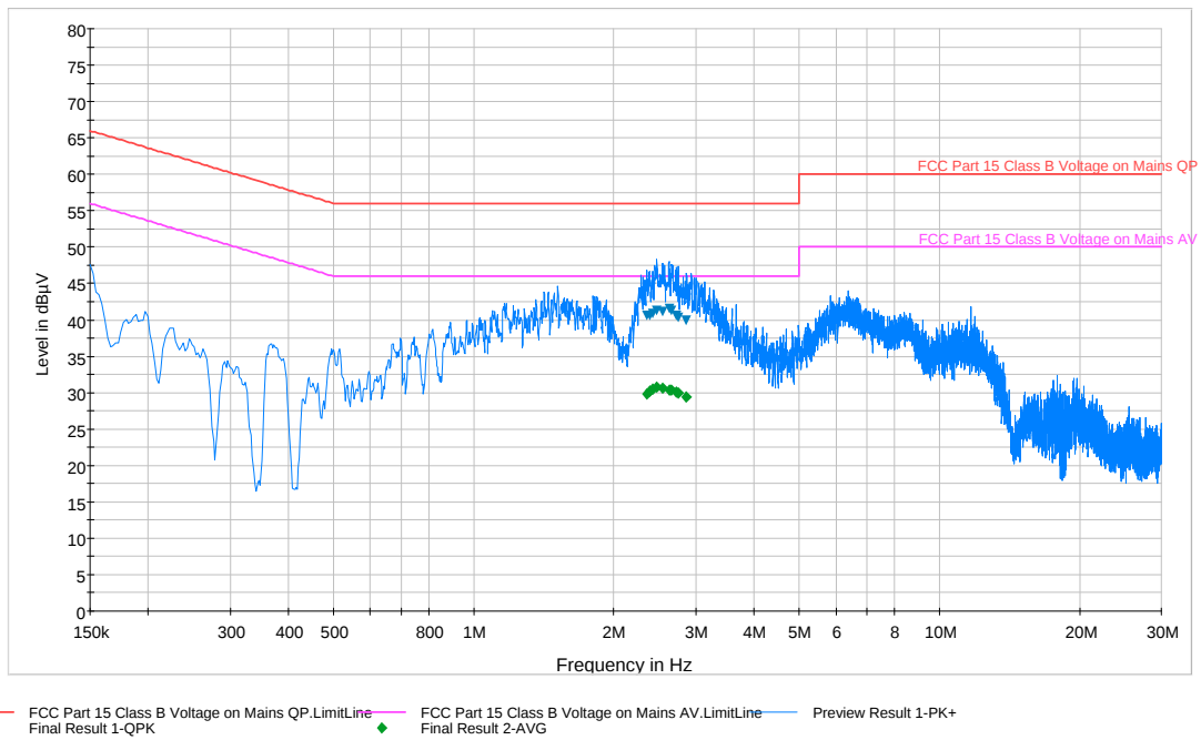
Plot 6-79. Line Conducted Plot with 802.11a (UNII Band 2) (LN)
