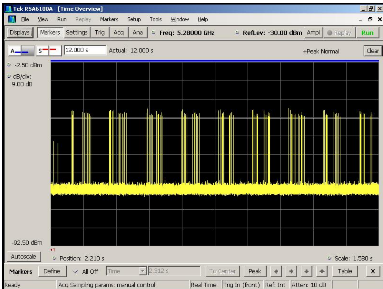
Figure 5-7. Aggregate Time (UNII Band 2)
