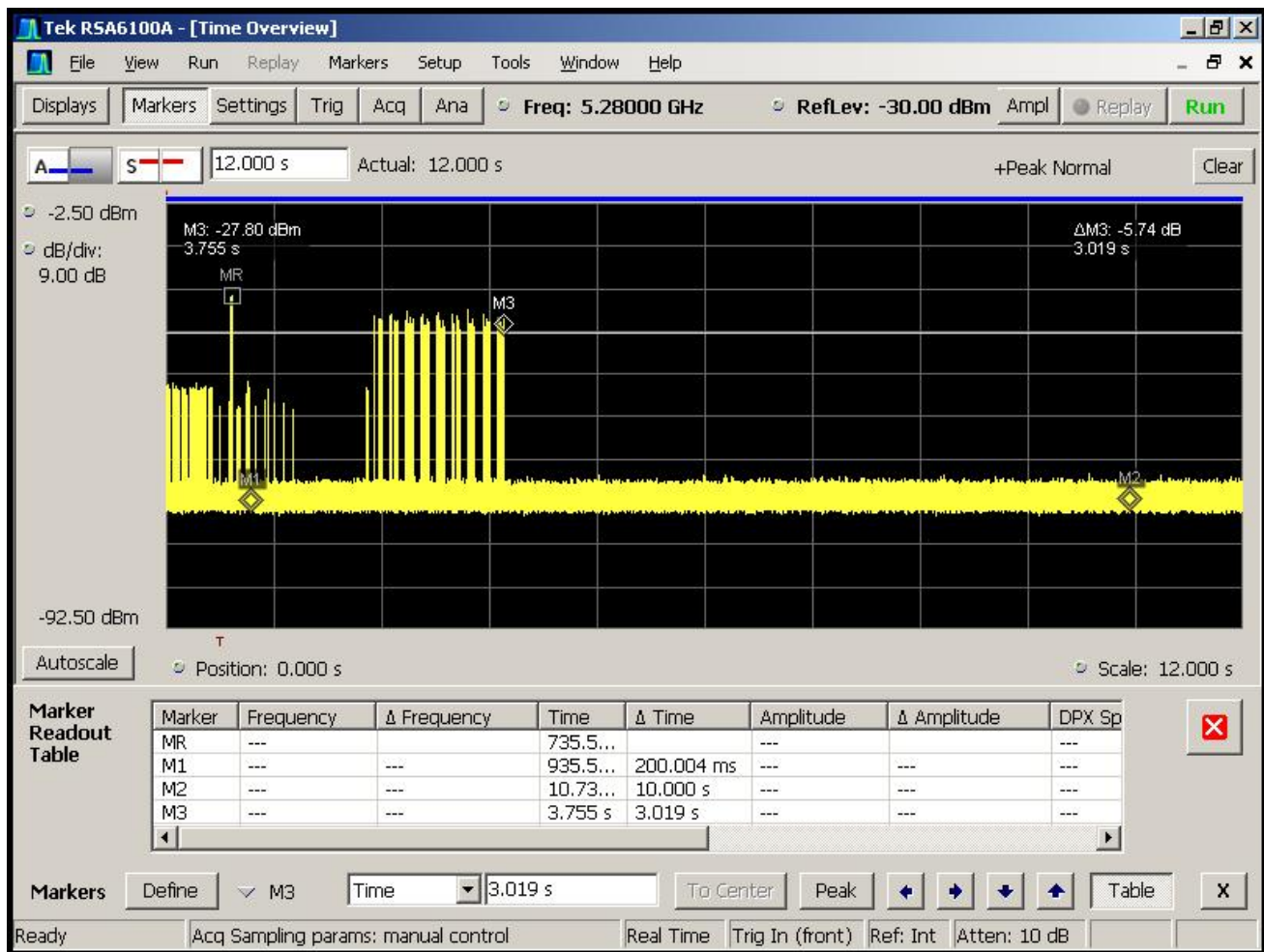
Figure 5-6. Channel Move Time (< 10sec)
