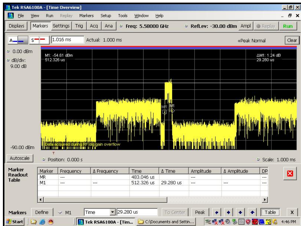
Figure 6-4. Pulse Width After 200ms
