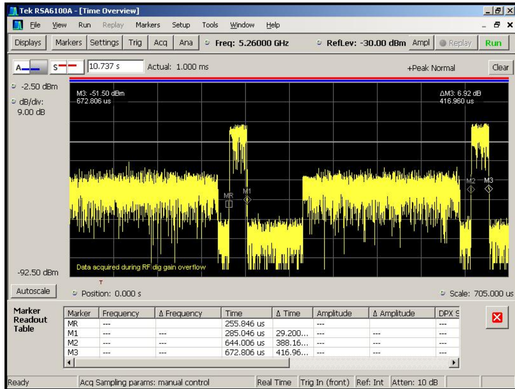
Figure 5-5. Pulse Width after 200ms
