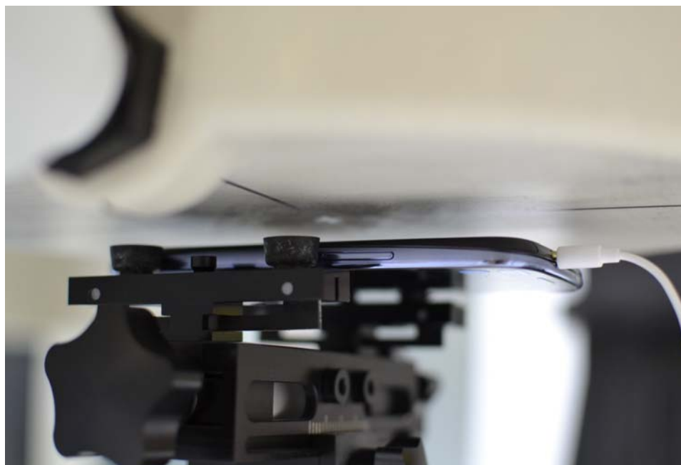
SAR Test Setup Photo 11 – Back Side Body-worn at 1.0 cm
