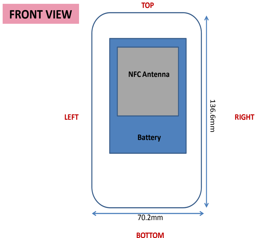
Figure 1-2 NFC Antenna Locations
