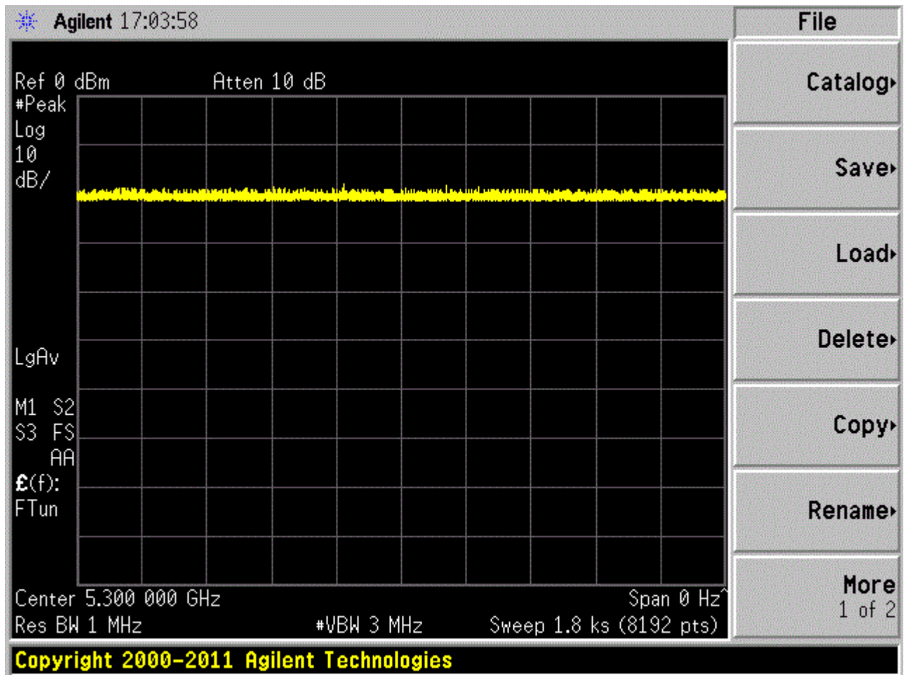
Figure 5-7 Non-occupancy Period - Monitoring live spectrum - Elapse time 30 minutes
