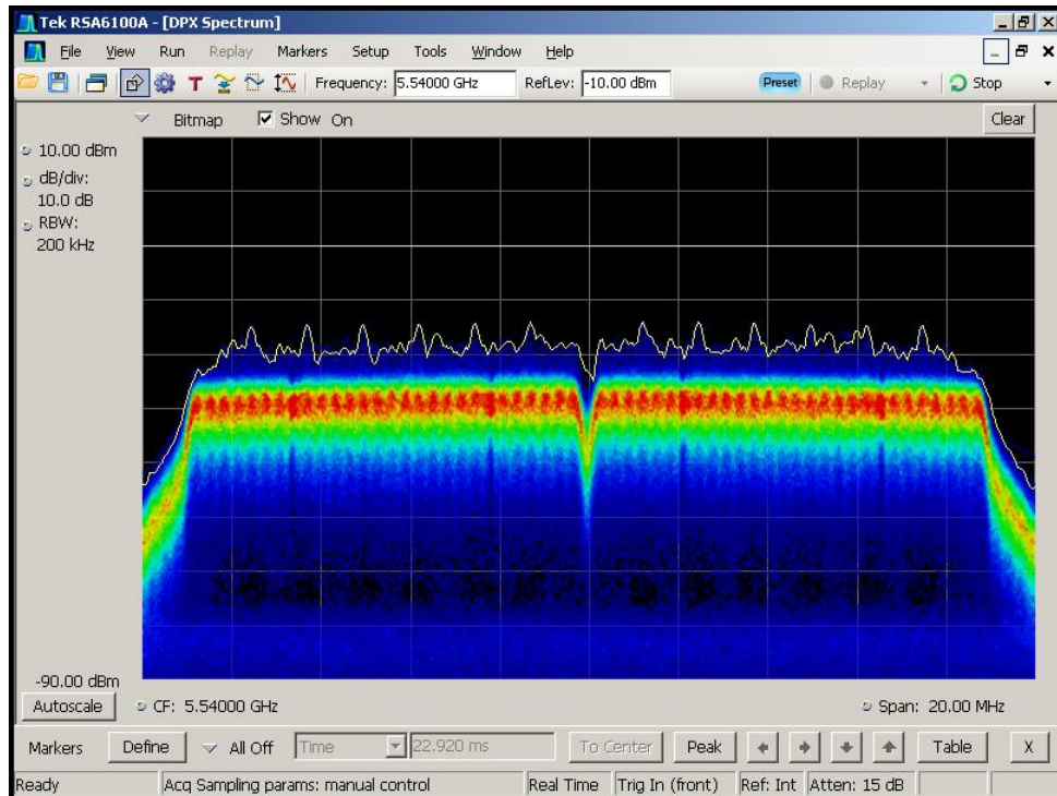
Figure 6-4. Real-Time Spectrum Display, WLAN Traffic (Streaming Video)
