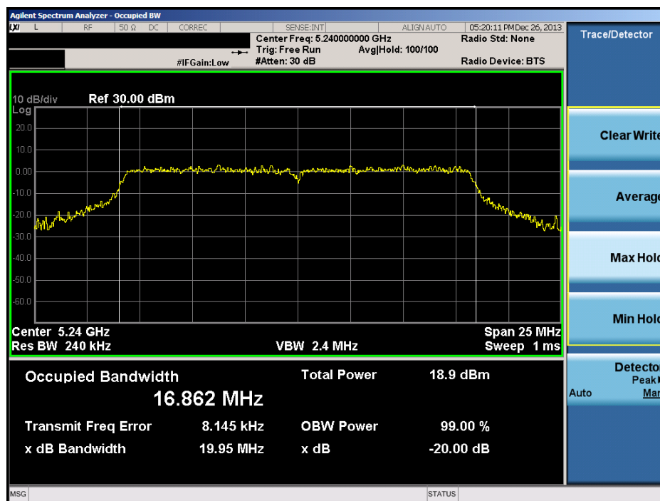
Plot 6-26. 20 dB Bandwidth Plot (802.11a (UNII Band 1) – Ch. 48)
