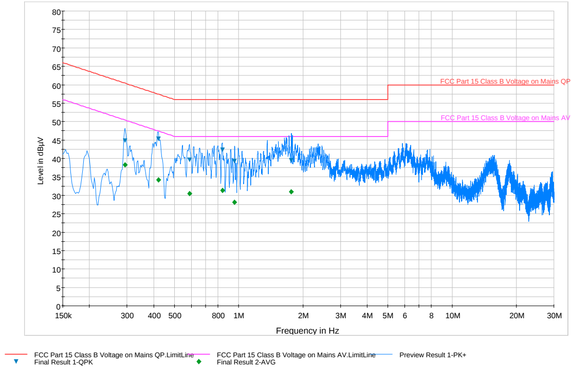
Plot 6-75. Line Conducted Plot with 802.11a UNII Band 3 (L1)
