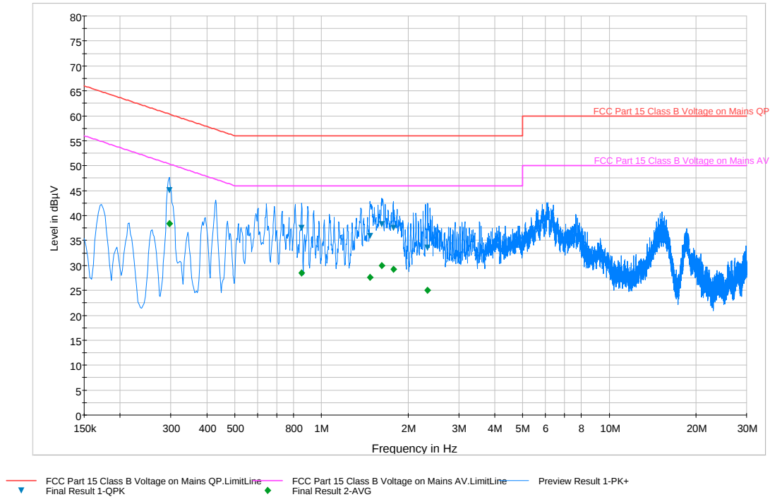
Plot 6-76. Line Conducted Plot with 802.11a UNII Band 3 (N)
