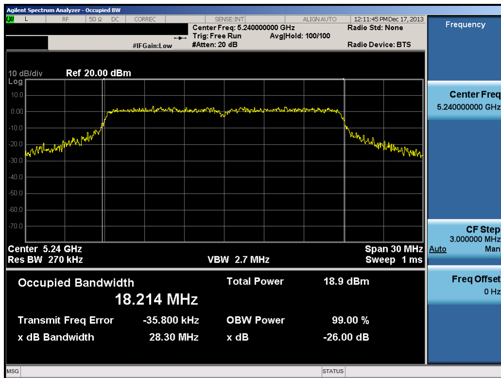
Plot 6-6. 26dB Bandwidth Plot (20MHz BW 802.11a/n (UNII Band 1) – Ch. 48)
