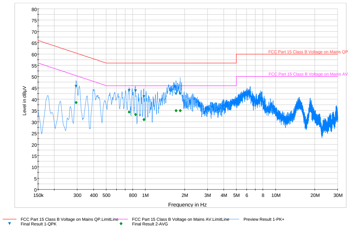
Plot 6-73. Line Conducted Plot with 802.11a UNII Band 2 (L1)
