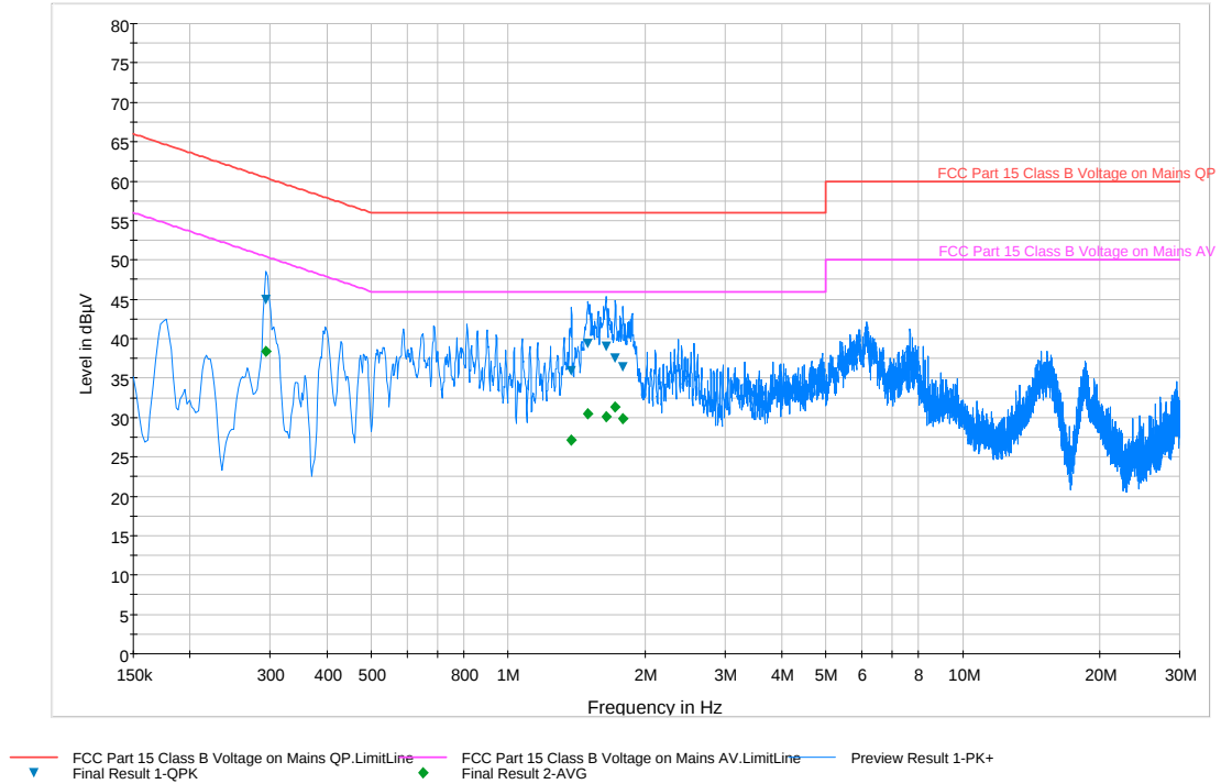
Plot 6-74. Line Conducted Plot with 802.11a UNII Band 2 (N)
