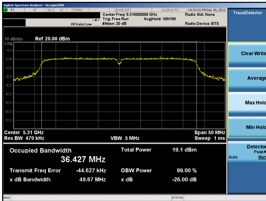
Plot 6-16. 26dB Bandwidth Plot (40MHz BW 802.11a/n (UNII Band 2A) – Ch. 62)
