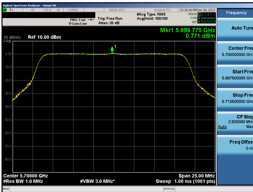
Plot 6-50. Peak Power Spectral Density Plot (20MHz BW 802.11a/n (UNII Band 3) – Ch. 140)
