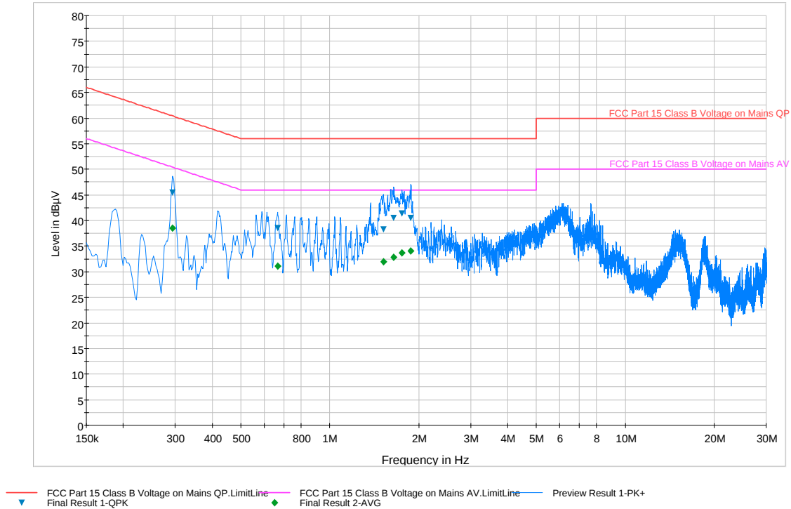
Plot 6-72. Line Conducted Plot with 802.11a UNII Band 1 (N)
