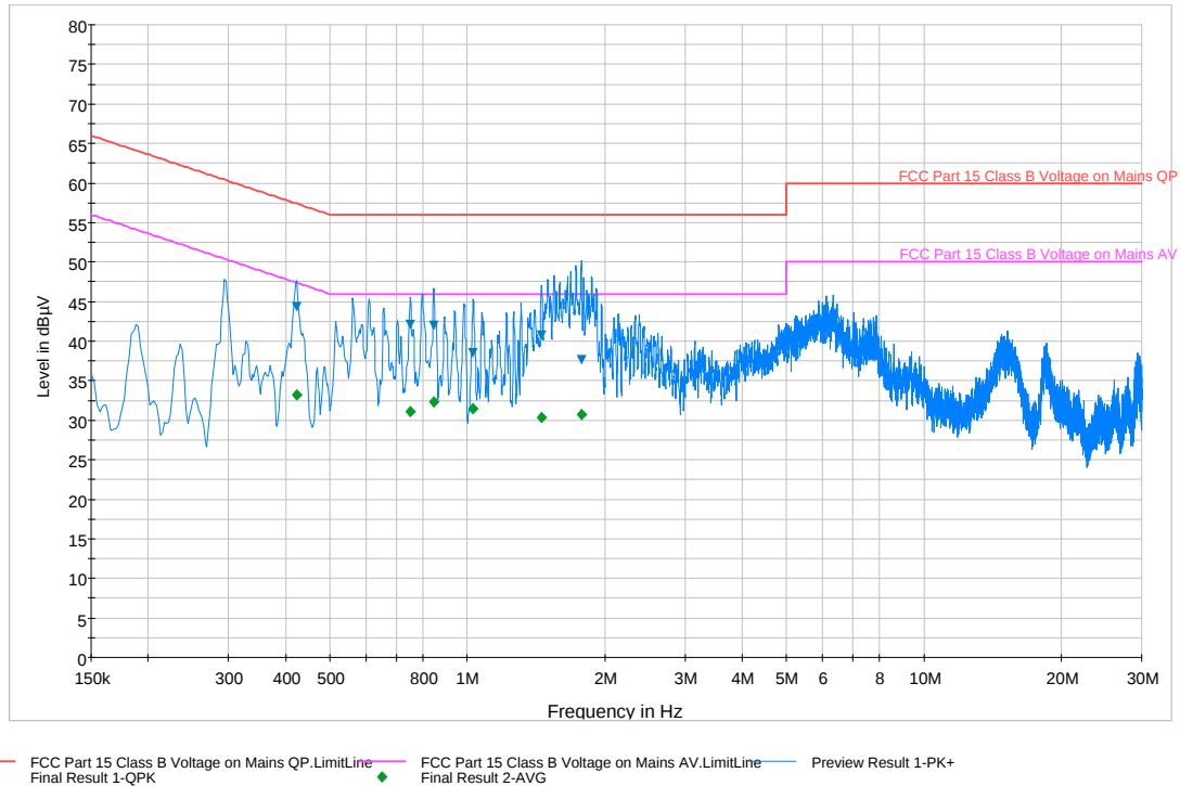
Plot 6-71. Line Conducted Plot with 802.11a UNII Band 1 (L1)
