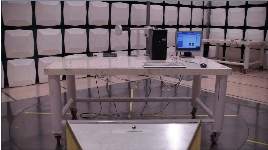
[ Radiated Disturbance for Above 1 GHz – Front ]
