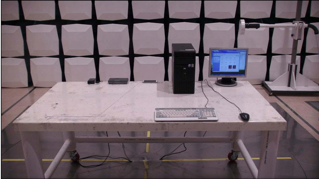
[ Radiated Disturbance for Below 1 GHz – Front ]
