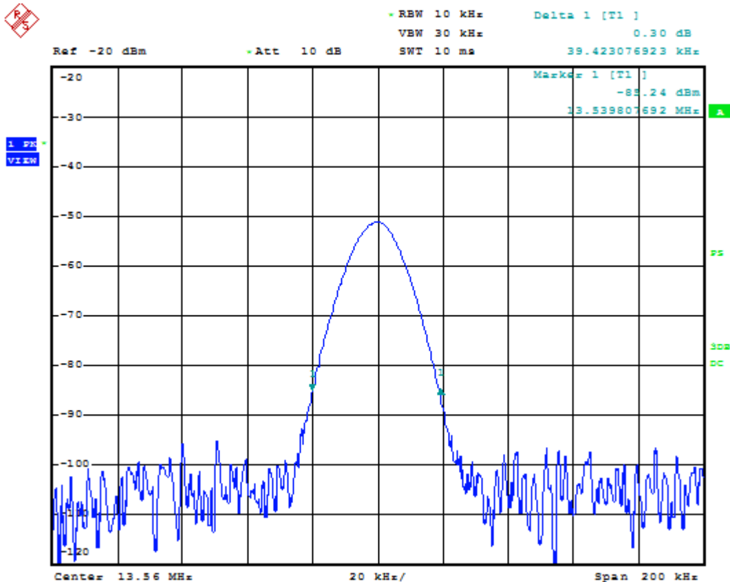
Figure 8-2. 20dB Bandwidth Plot
