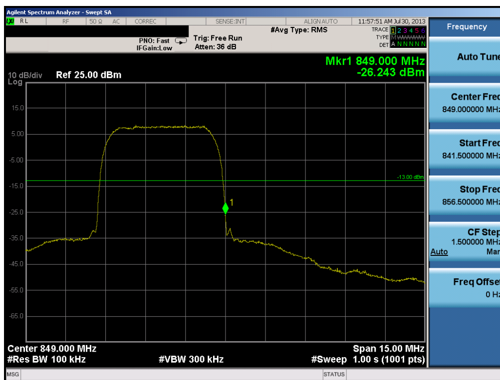
Plot 6-39. Band Edge Plot (Cellular WCDMA Mode – Ch. 4233)
