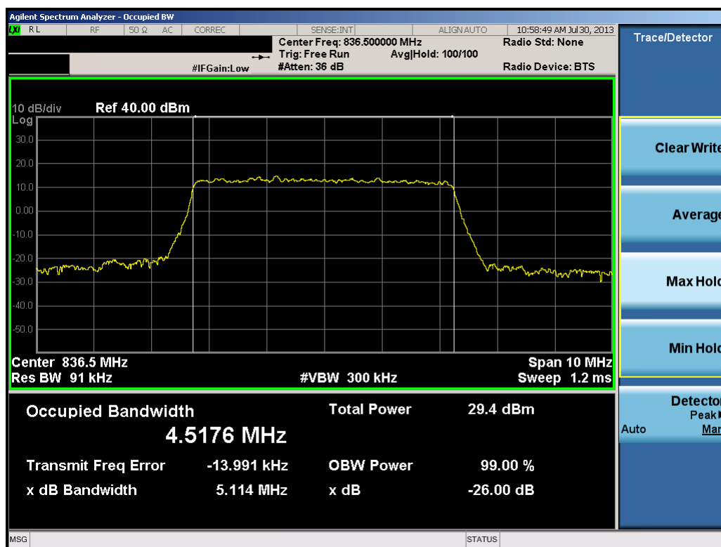
Plot 7-23. Occupied Bandwidth Plot (5.0MHz 16-QAM – RB Size 25)
