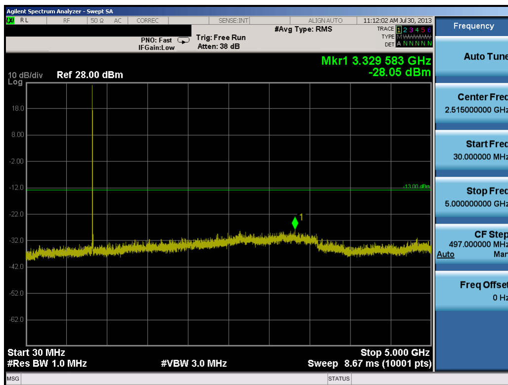
Plot 7-28. Conducted Spurious Plot (5.0MHz QPSK – RB Size 1, RB Offset 0 – High Channel)
