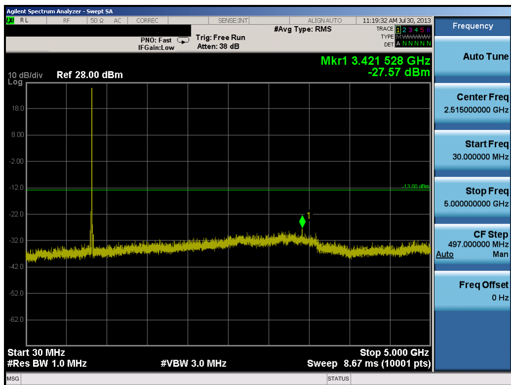
Plot 7-38. Conducted Spurious Plot (10.0MHz QPSK – RB Size 1, RB Offset 0 – High Channel)
