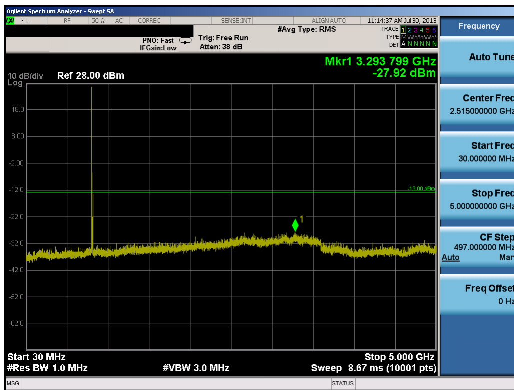
Plot 7-34. Conducted Spurious Plot (10.0MHz QPSK – RB Size 1, RB Offset 0– Low Channel)
