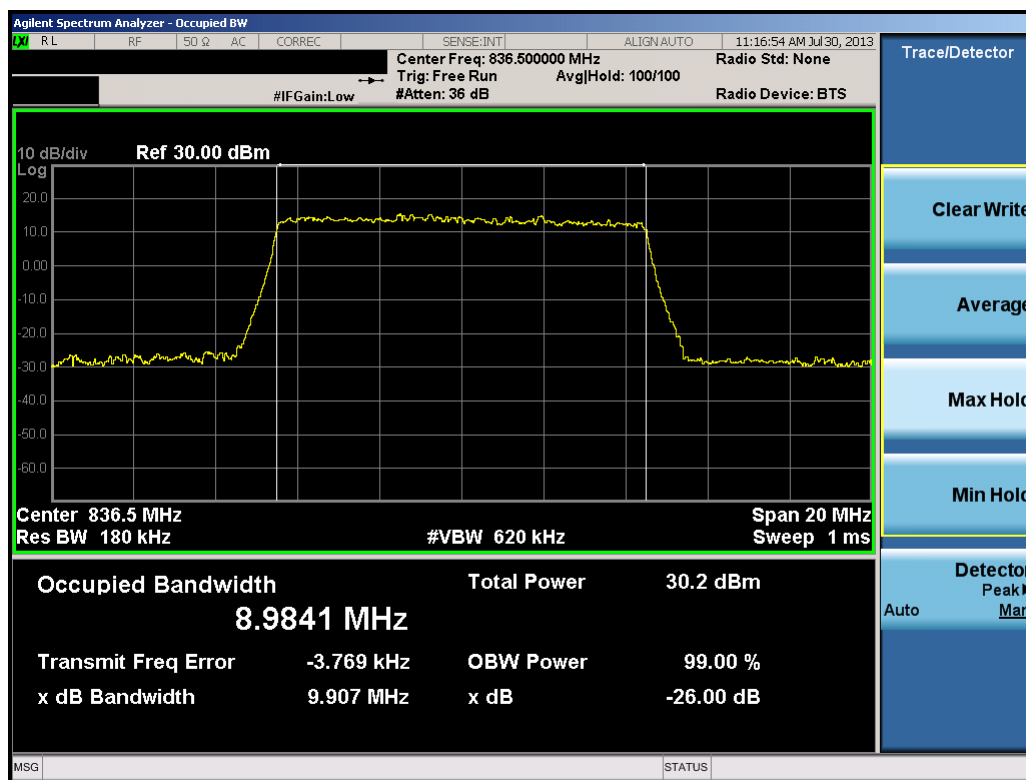
Plot 7-32. Occupied Bandwidth Plot (10.0MHz QPSK – RB Size 50)
