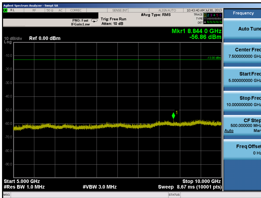
Plot 7-17. Conducted Spurious Plot (3.0MHz QPSK – RB Size 1, RB Offset 0 – Mid Channel)
