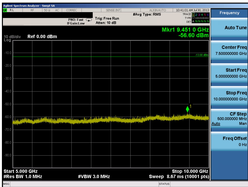
Plot 7-15. Conducted Spurious Plot (3.0MHz QPSK – RB Size 1, RB Offset 0 – Low Channel)
