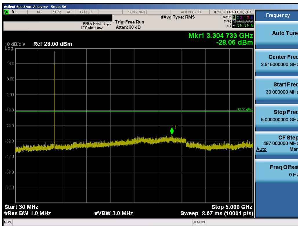
Plot 7-18. Conducted Spurious Plot (3.0MHz QPSK – RB Size 1, RB Offset 0 – High Channel)
