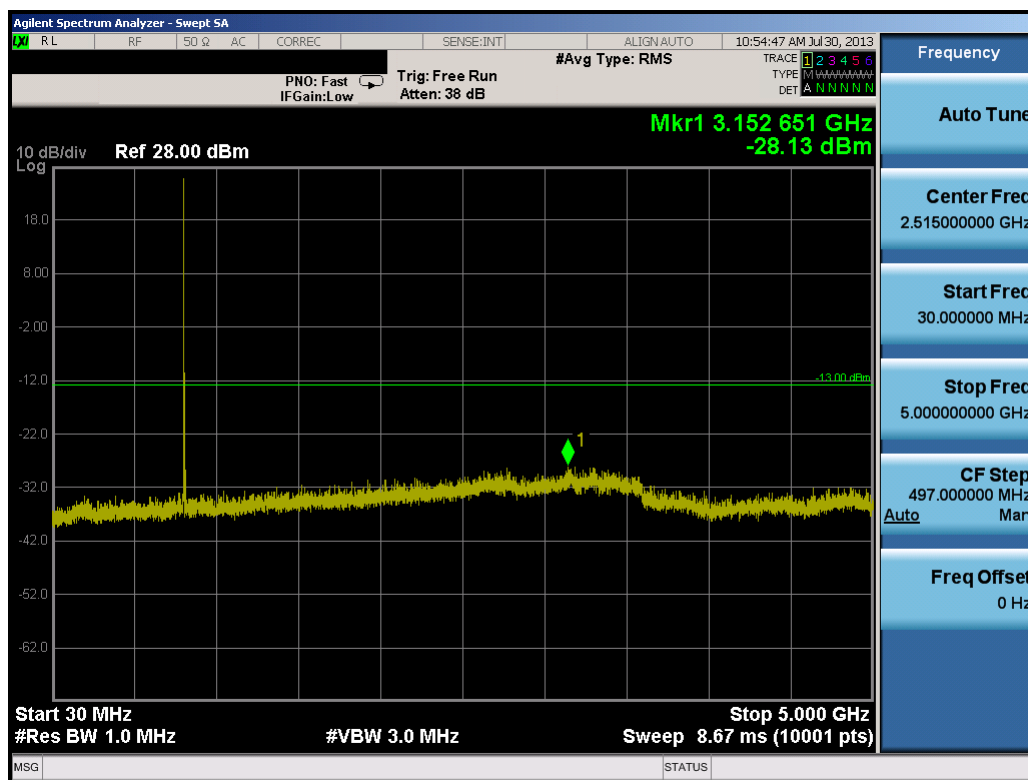
Plot 7-24. Conducted Spurious Plot (5.0MHz QPSK – RB Size 1, RB Offset 0 – Low Channel)
