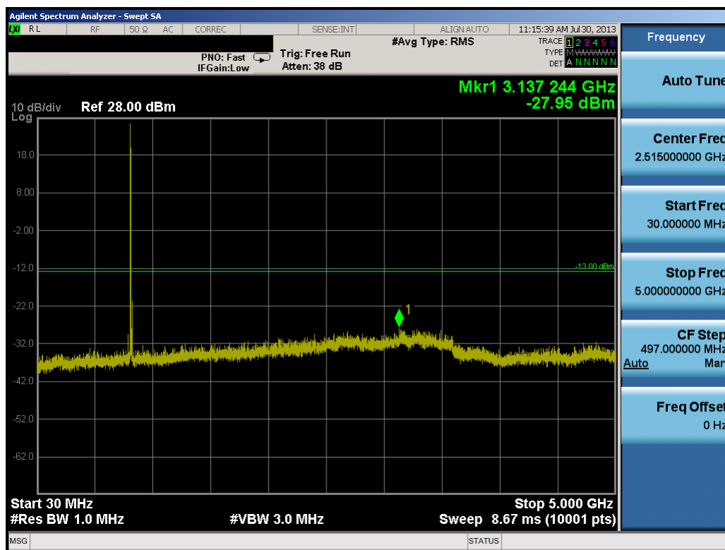
Plot 7-36. Conducted Spurious Plot (10.0MHz QPSK – RB Size 1, RB Offset 0 – Mid Channel)
