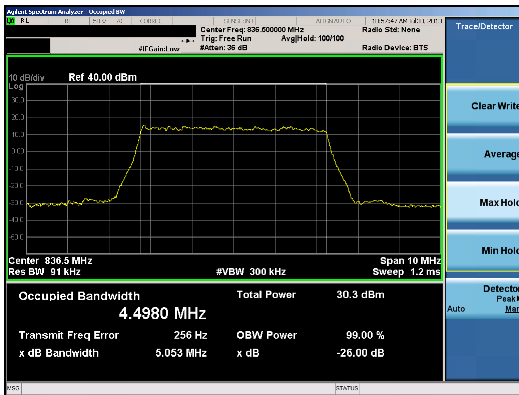
Plot 7-22. Occupied Bandwidth Plot (5.0MHz QPSK – RB Size 25)
