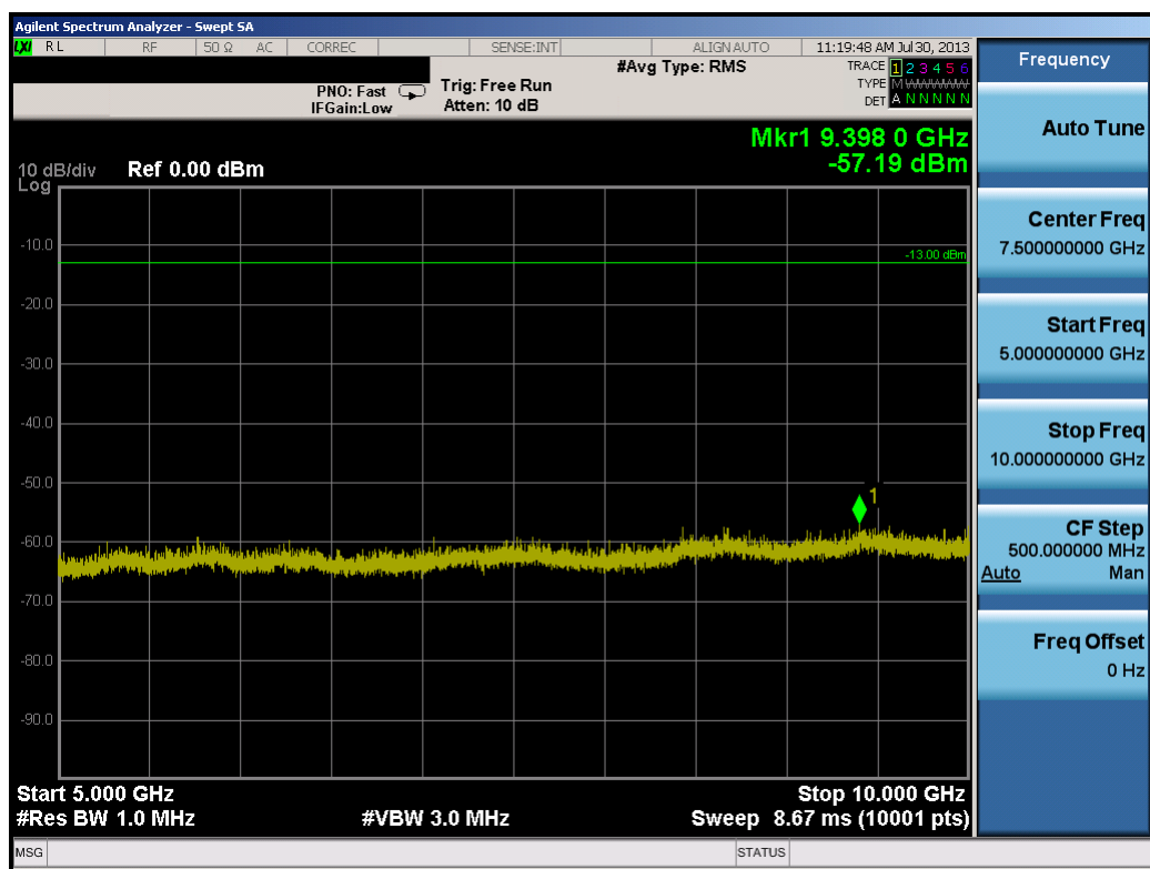
Plot 7-39. Conducted Spurious Plot (10.0MHz QPSK – RB Size 1, RB Offset 0 – High Channel)
