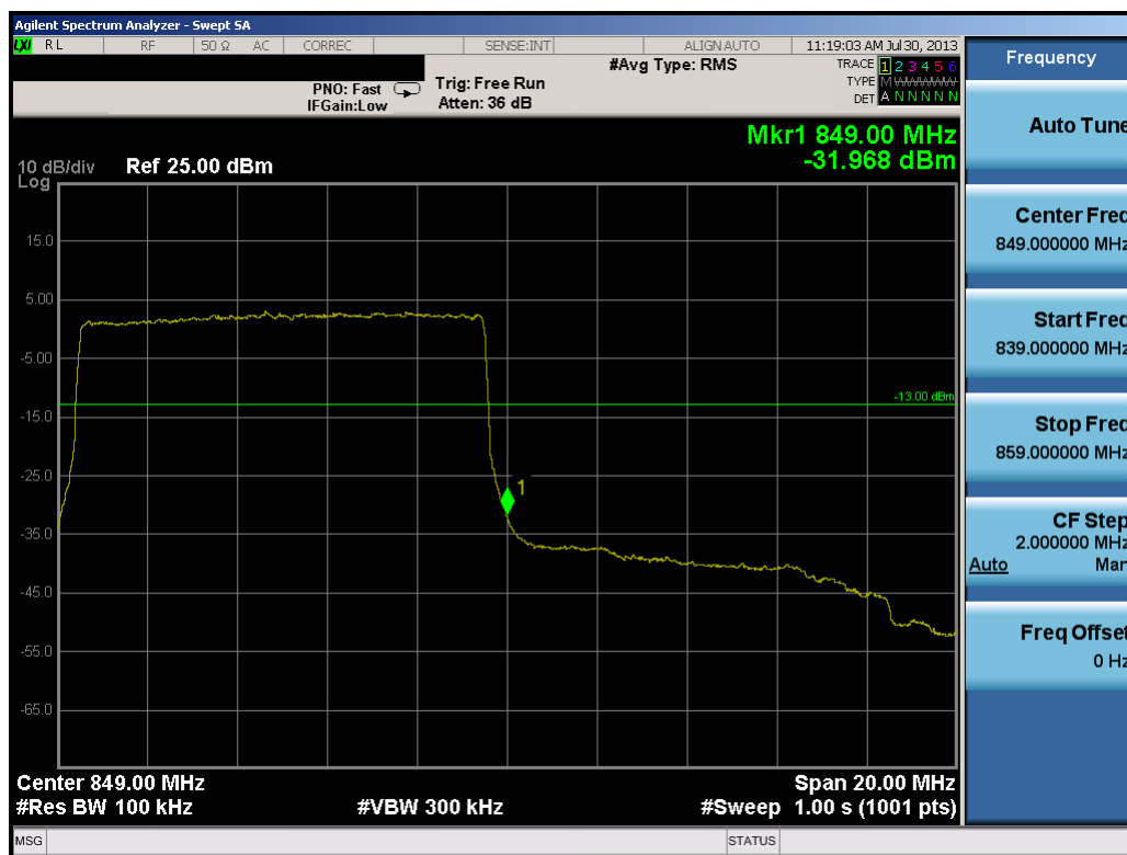
Plot 7-40. Upper Band Edge Plot (10.0MHz QPSK – RB Size 50)
