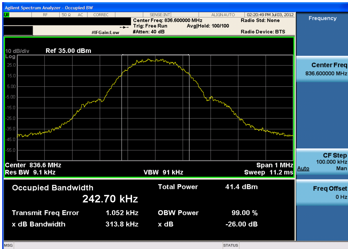
Plot 7-8. Occupied Bandwidth Plot (Cellular GSM Mode – Ch. 190)
