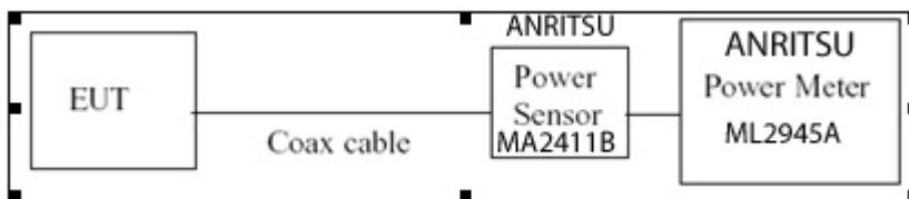
Figure 6-3. Test Instrument & Measurement Setup
