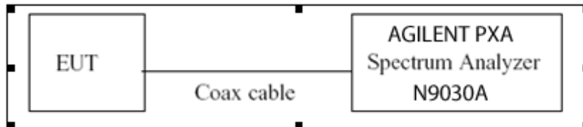
Figure 6-4. Test Instrument & Measurement Setup
