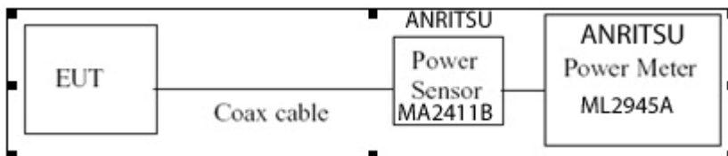
Figure 6-2. Test Instrument & Measurement Setup
