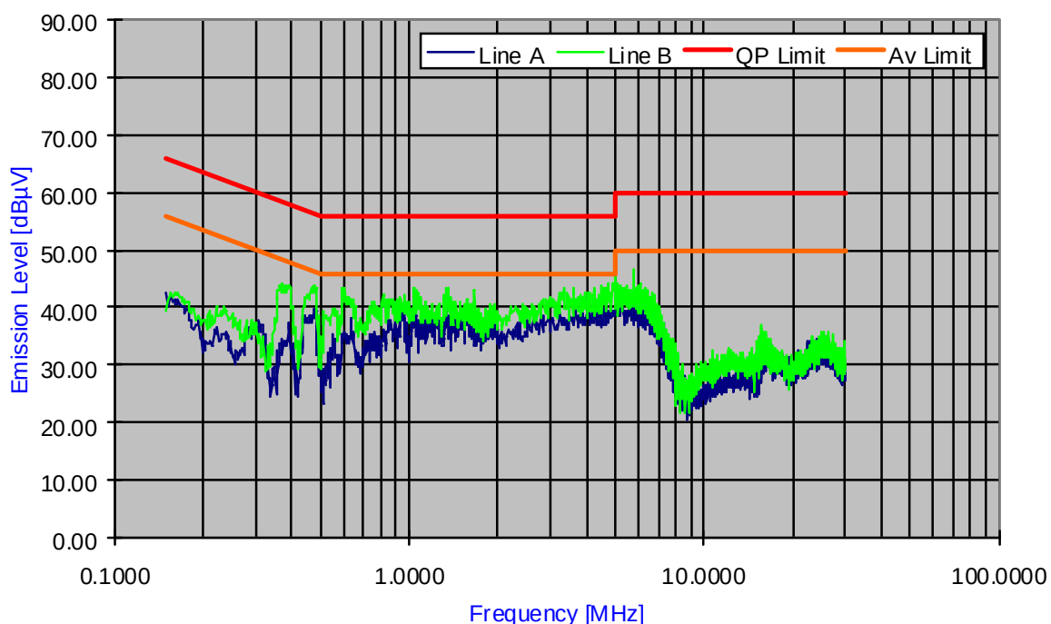
Plot 6-56. Line Conducted Plot with 802.11b
