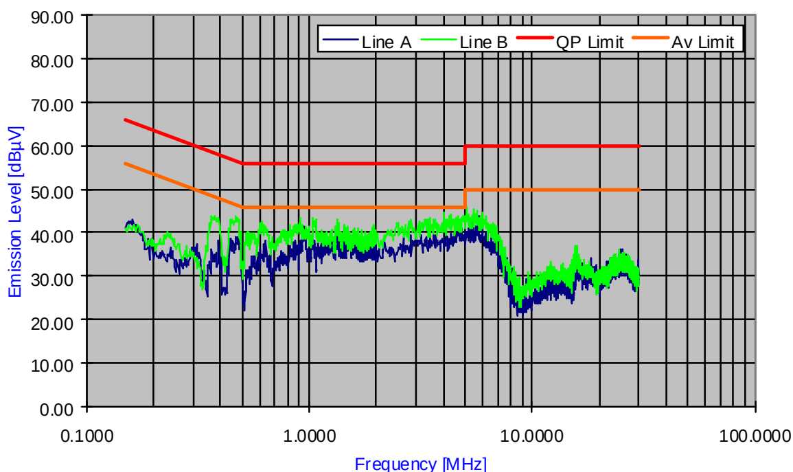
Plot 6-57. Line Conducted Plot with 802.11a
